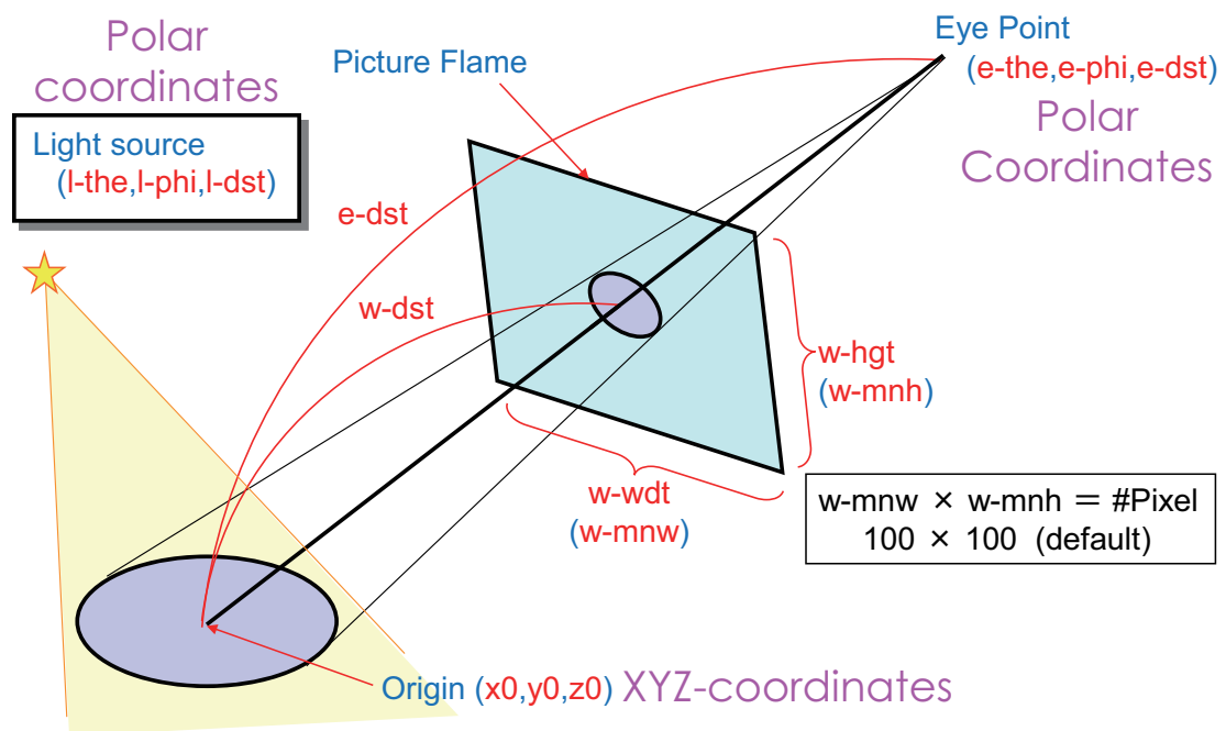
Figure 6.7: 3dshow tally: origin ( x_0, y_0, z_0 ), eye point ( e\text{-the}, e\text{-phi}, e\text{-dst} ), light source ( l\text{-the}, l\text{-phi}, l\text{-dst} ), and picture plane ( w\text{-wdt}, w\text{-hgt}, w\text{-dst} ).
