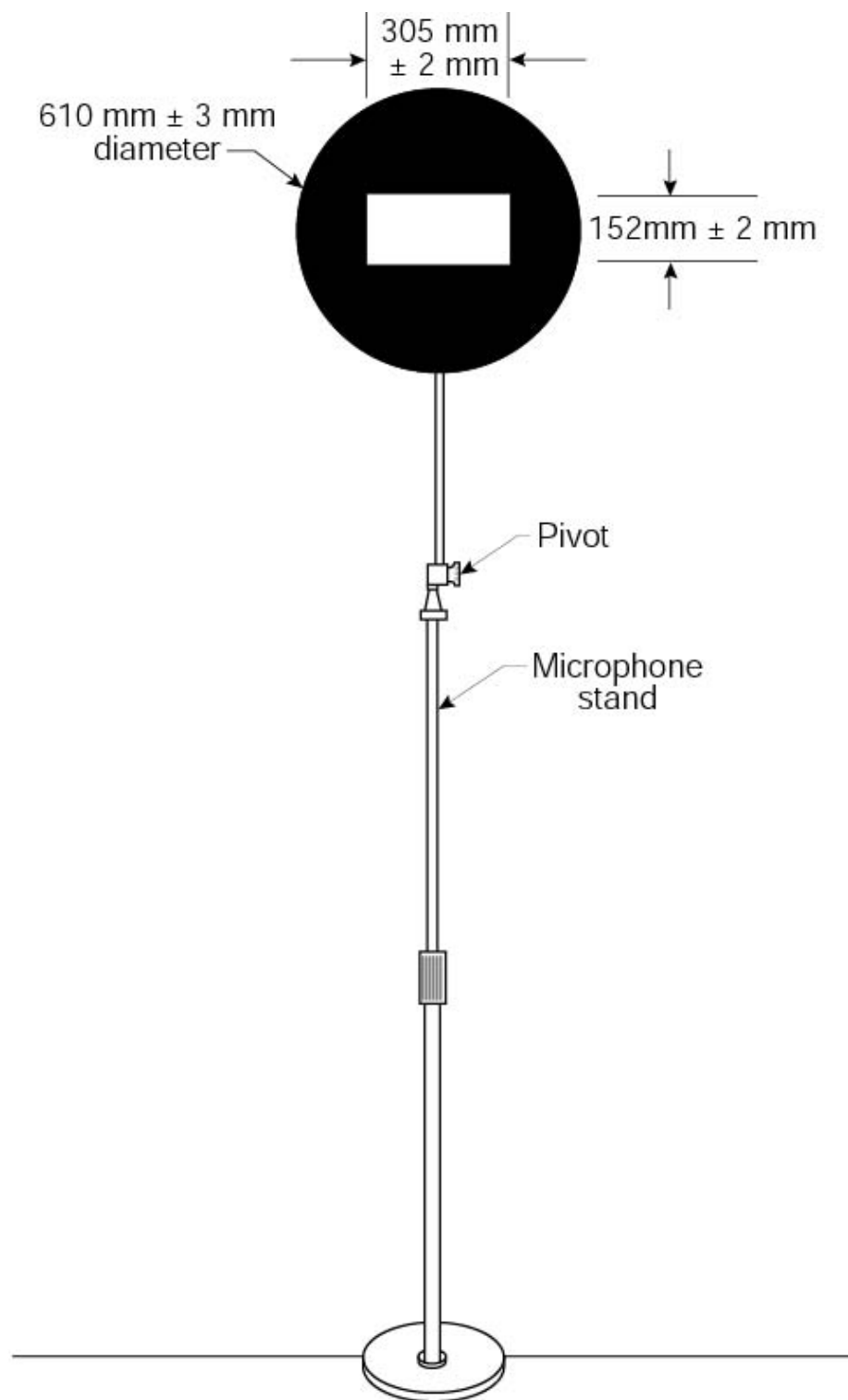
Figure 6. Schematic of the long-range target apparatus
