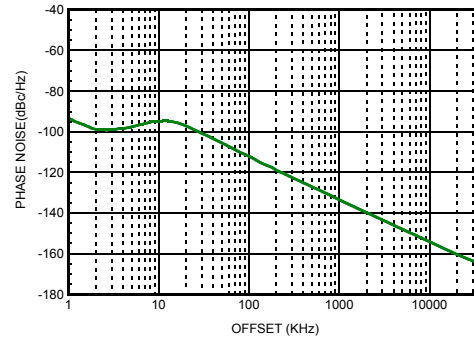
Figure 36. HMC835LP6GE with External VCO HMC384LP4E at 2213MHz [25]
