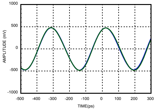
Figure 25. Phase Adjust at 0 degree [18]
