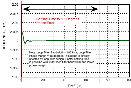
Figure 33. Frequency Settling After Frequency Change, Manual Calibration [23]
