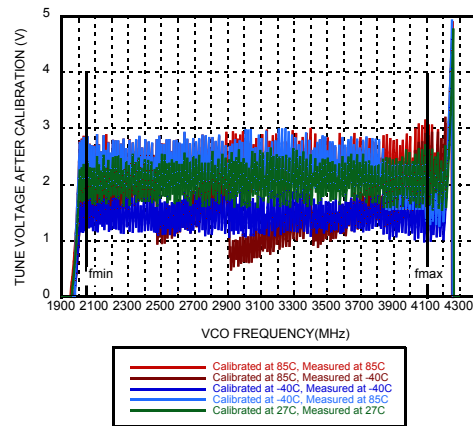
Figure 10. Typical Tuning Voltage After Calibration [6]
