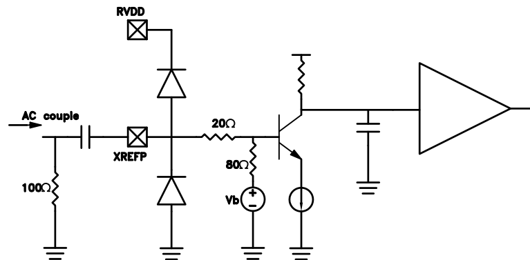
Figure 43. Reference Path Input Stage
