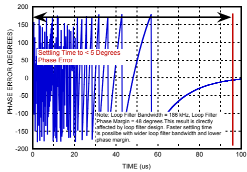
Figure 32. Phase Settling After Frequency Change, AutoCal Enabled [22]
