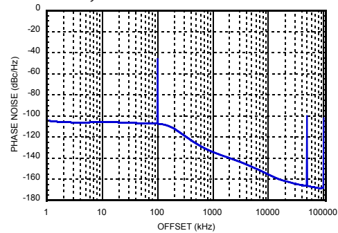
Figure 20. Typical Spurious Emissions at 3000.1 MHz, Fixed Reference [14]
