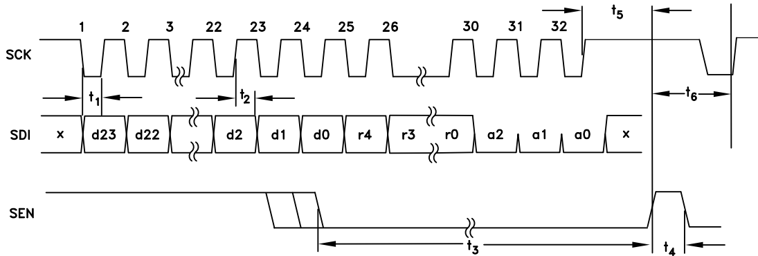
Figure 45. Serial Port Timing Diagram - WRITE
