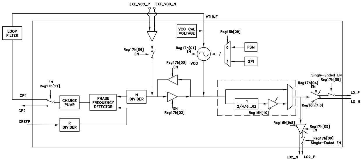
Figure 39. HMC835LP6GE PLL VCO Block Diagram
