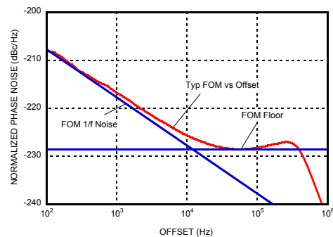
Figure 28. Figure of Merit
