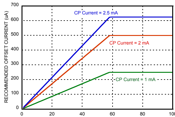
Recommended CP offset current vs PD frequency for typical CP gain currents. Calculated using (EQ 9)
