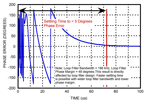
Figure 34. Phase Settling After Frequency Change, Manual Calibration [23]
