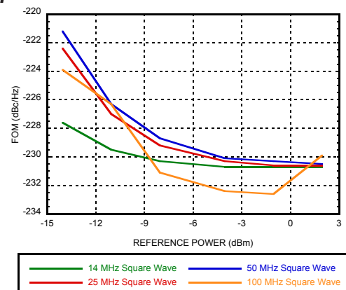
Figure 23. Reference Input Sensitivity, Square Wave [17]
