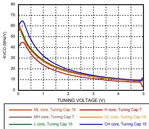
Figure 9. Typical VCO Sensitivity
