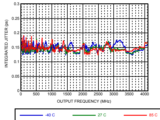
Figure 12. Single Sideband Integrated Phase Noise [7]
