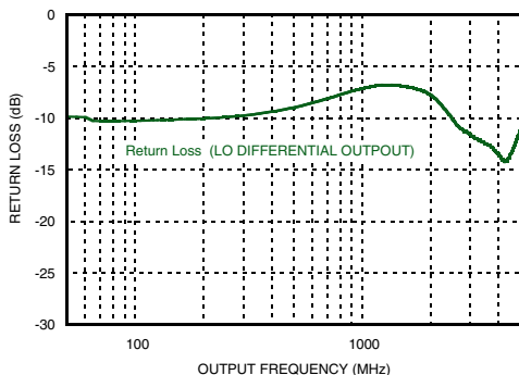
Figure 29. RF Output Return Loss Diff [21]
