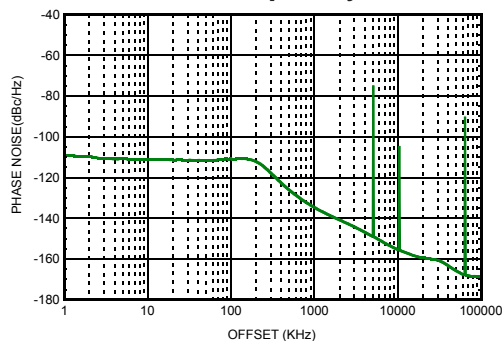
Figure 17. Fractional Spurious Performance at 2646.96 MHz, Exact Frequency Mode ON [11]
