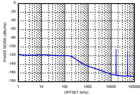
Figure 15. Fractional Spurious Performance at 904 MHz, Exact Frequency Mode ON [10]
