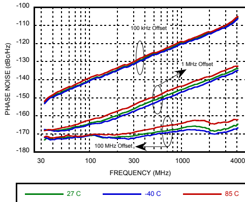
Figure 11. Open Loop Phase Noise vs. Temp
