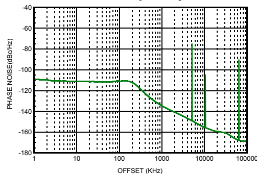
Figure 18. Fractional Spurious Performance at 2646.96 MHz, Exact Frequency Mode OFF [12]
