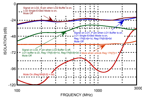
Figure 37. HMC835LP6GE Mute and Isolations
