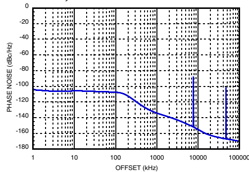
Figure 21. Typical Spurious Emissions at 3000.1 MHz, Tunable Reference [15]
