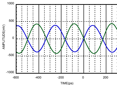
Figure 27. Phase Adjust at 180 degree [20]
