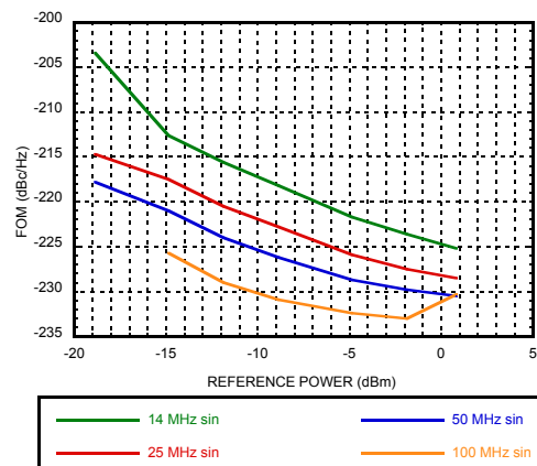
Figure 24. Reference Input Sensitivity, Sinusoidal Wave [17]
