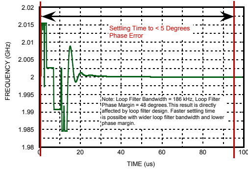
Figure 31. Frequency Settling After Frequency Change, AutoCal Enabled [22]
