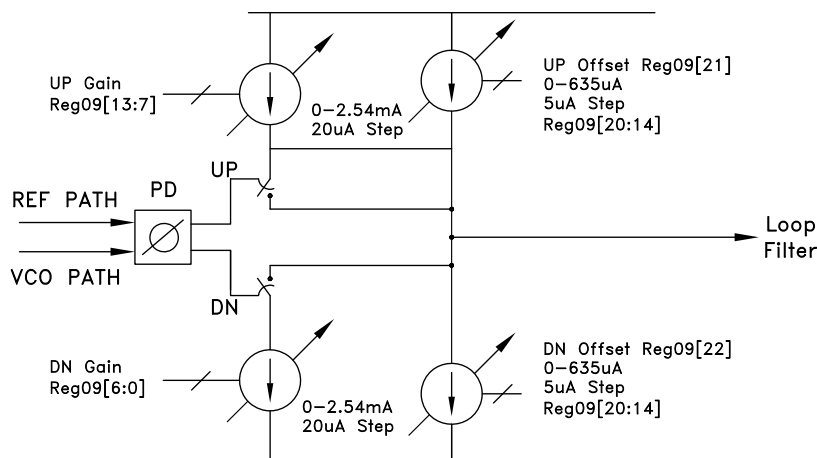
Figure 42. Charge Pump Gain & Offset Control
