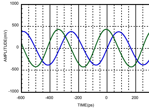
Figure 26. Phase Adjust at 90 degree [19]
