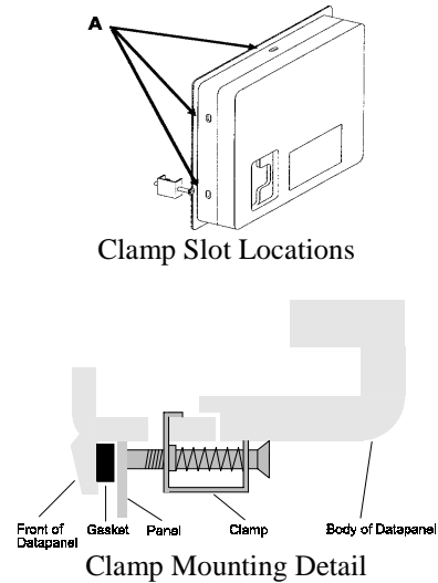
Figure 2-1. Datapanel Mounting Clamps
