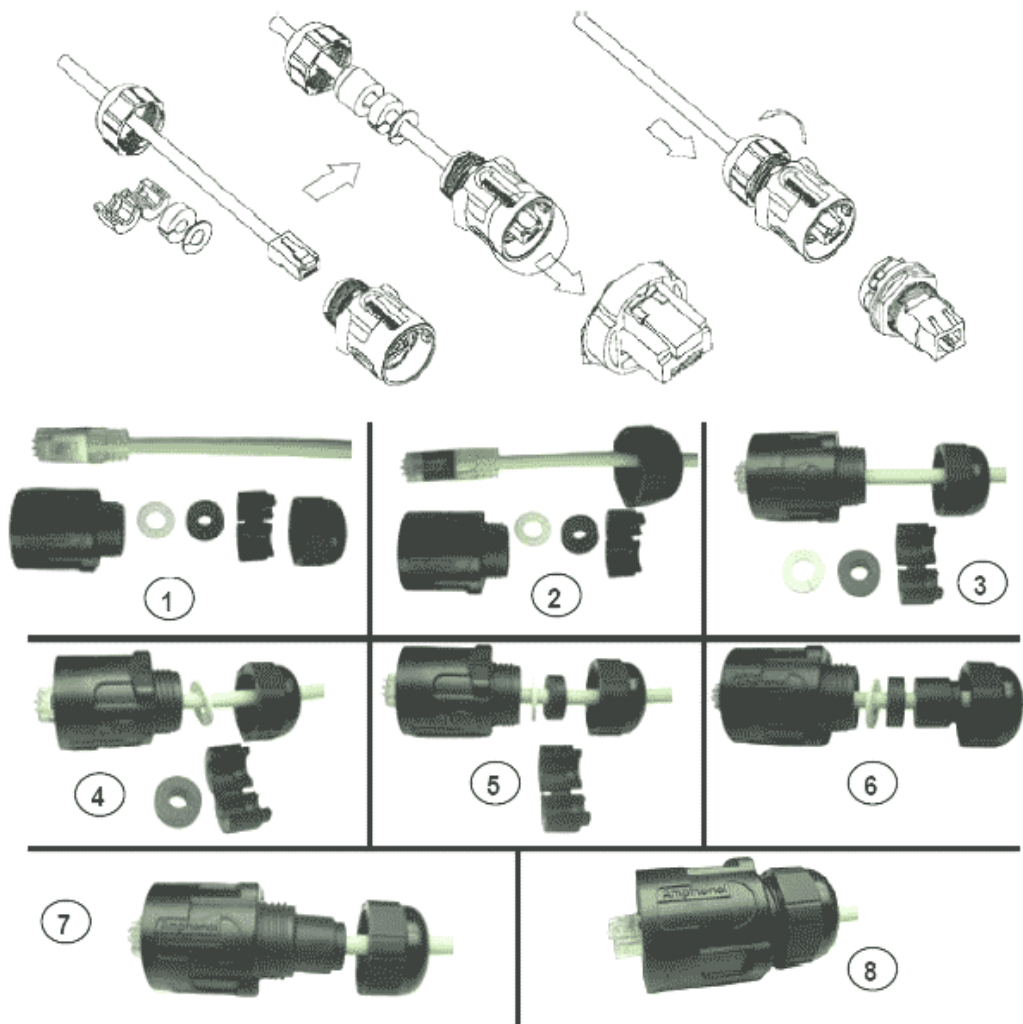
RJ45 Plug Assembly
