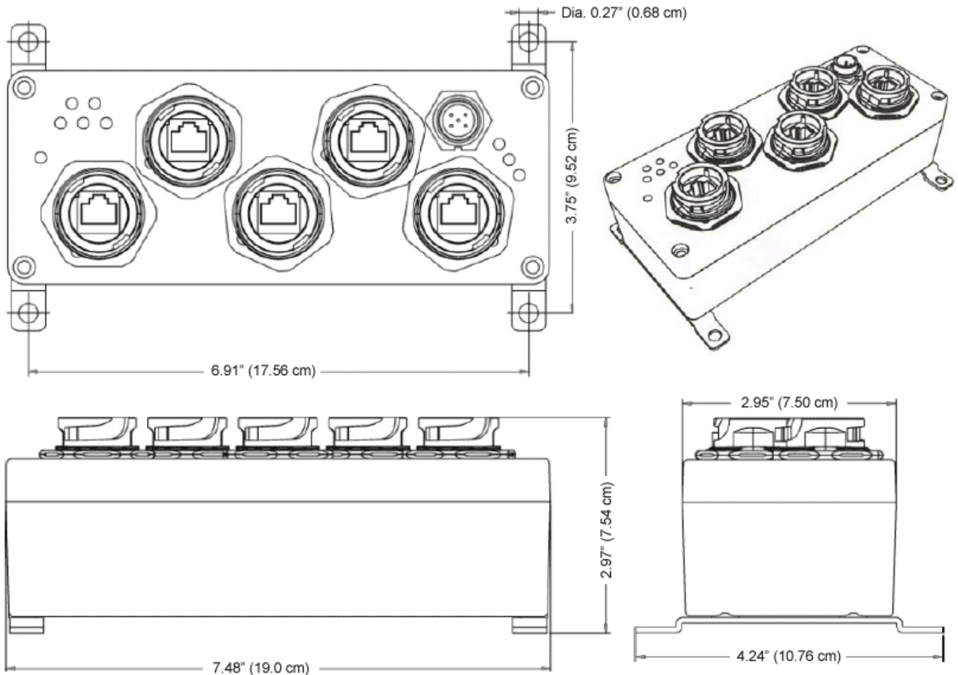
Switch Mechanical Dimensions
