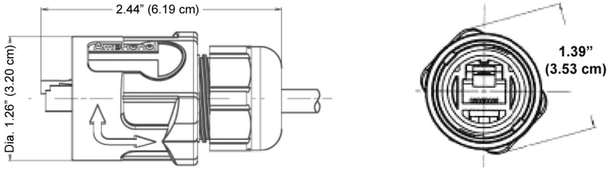
RJ45 Plug Mechanical Dimensions
