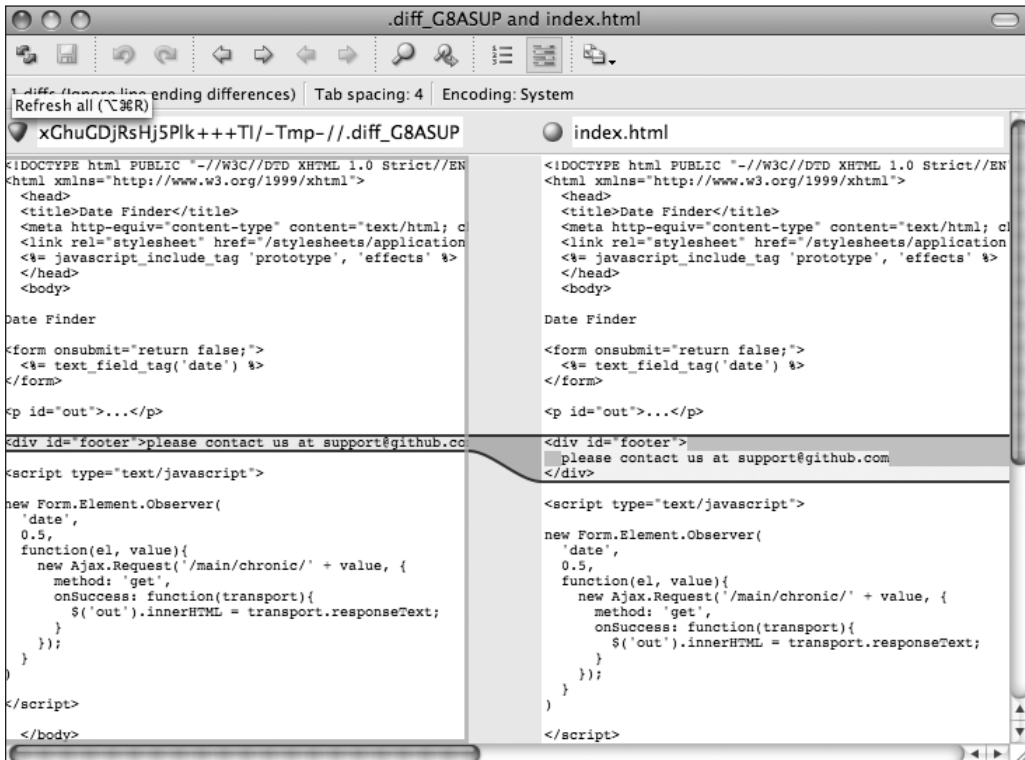
Figure 7-1. P4Merge
