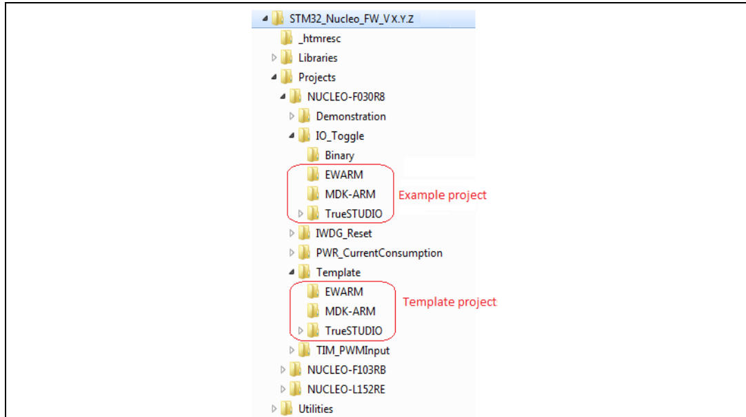
Figure 4. Package contents
