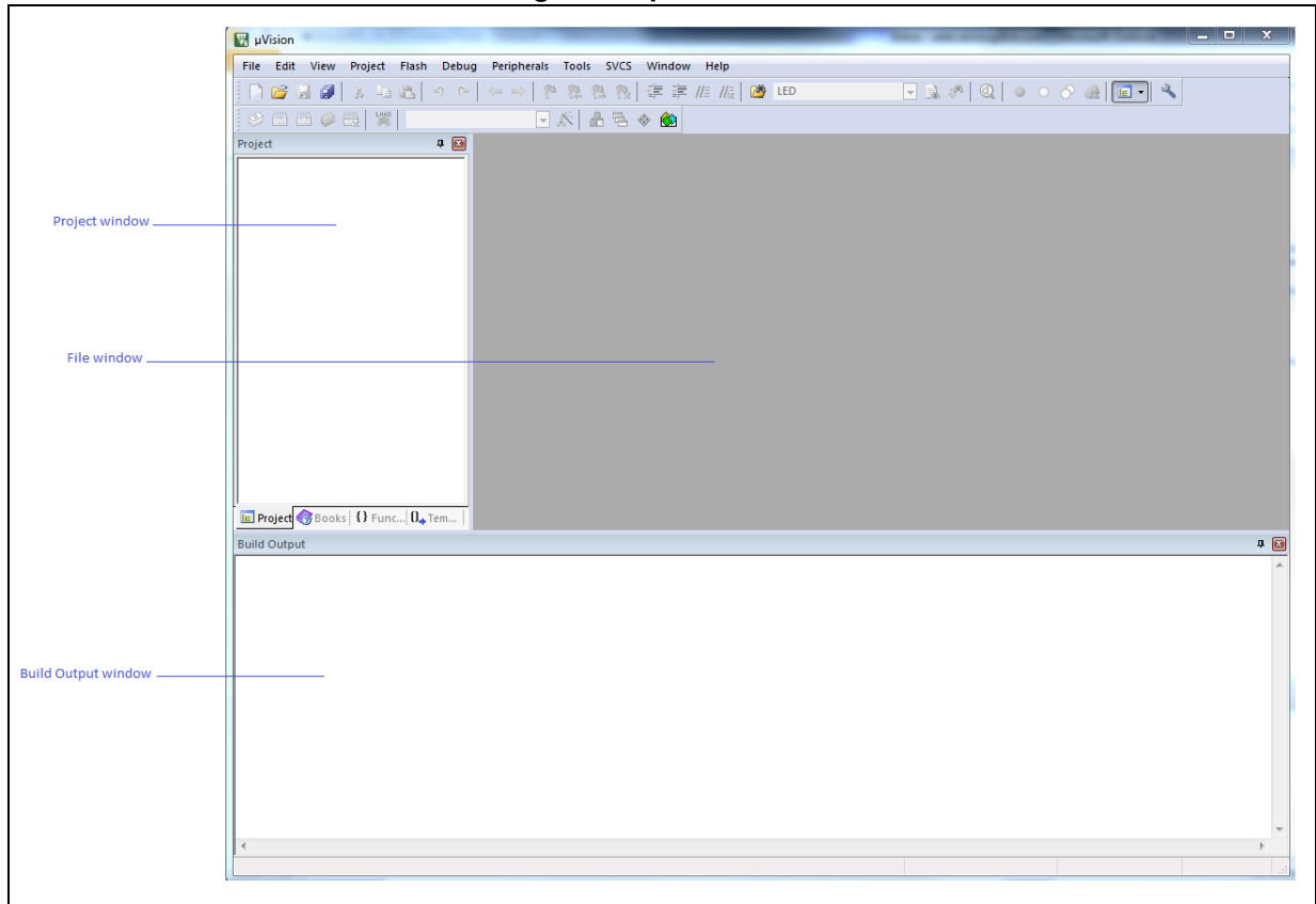
Figure 10. µvision5 IDE
