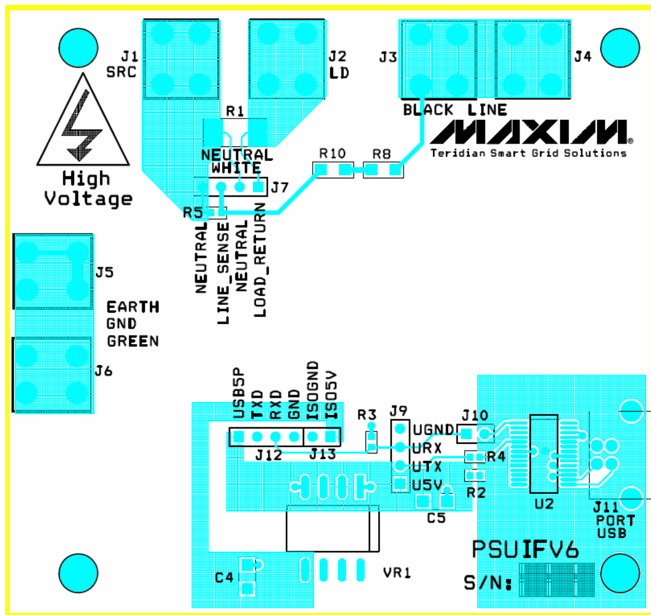
Figure 12: Shunt Adaptor Board PCB Top View
