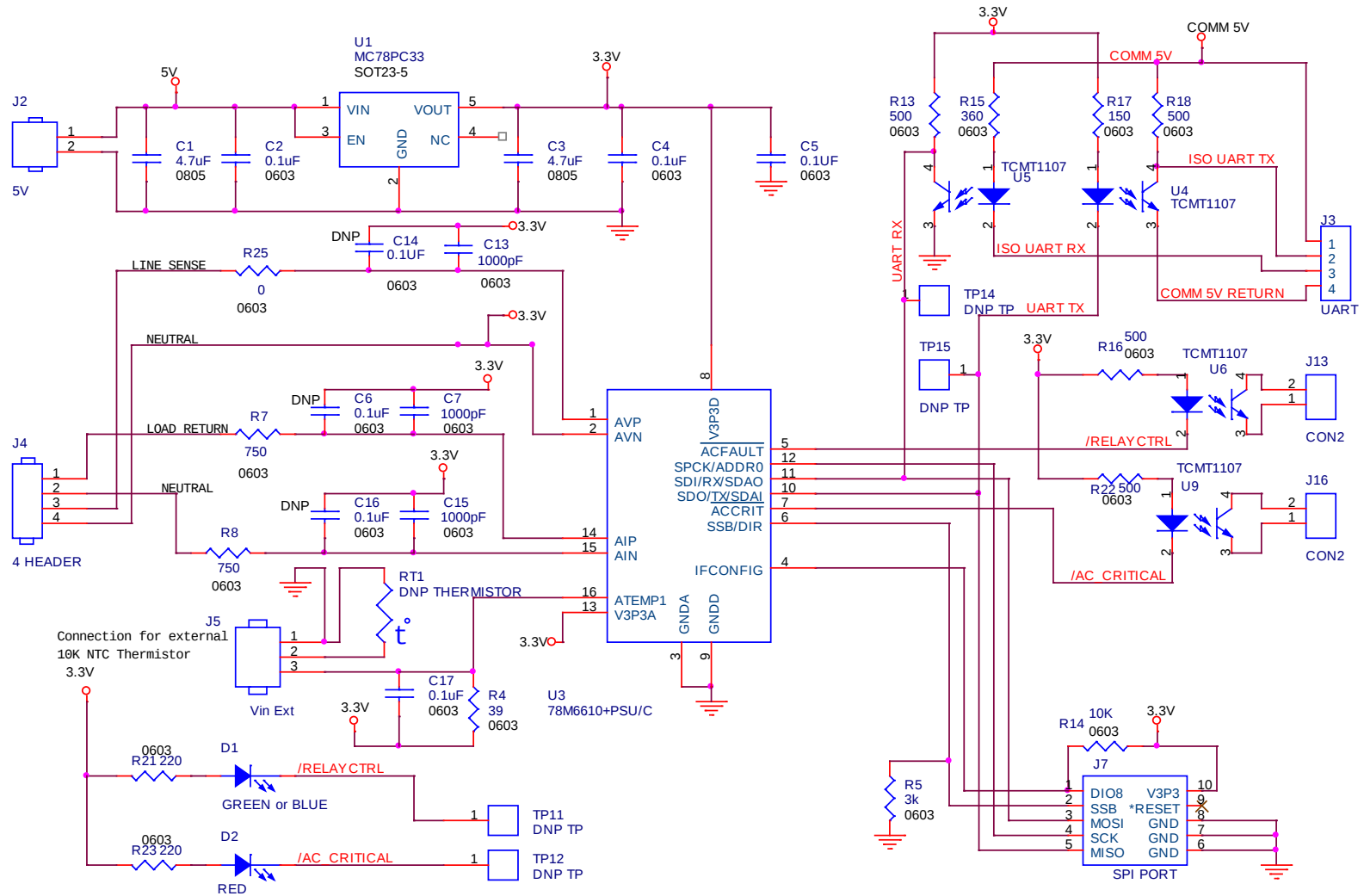
Figure 5: 78M6610+PSU 16-Pin Evaluation Board Electrical Schematic
