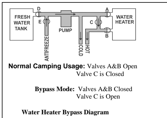
Factory installed water heater bypass
