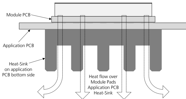
Figure 84: Thermal solution example providing a heat sink on the backside of the application board, below the cellular module
