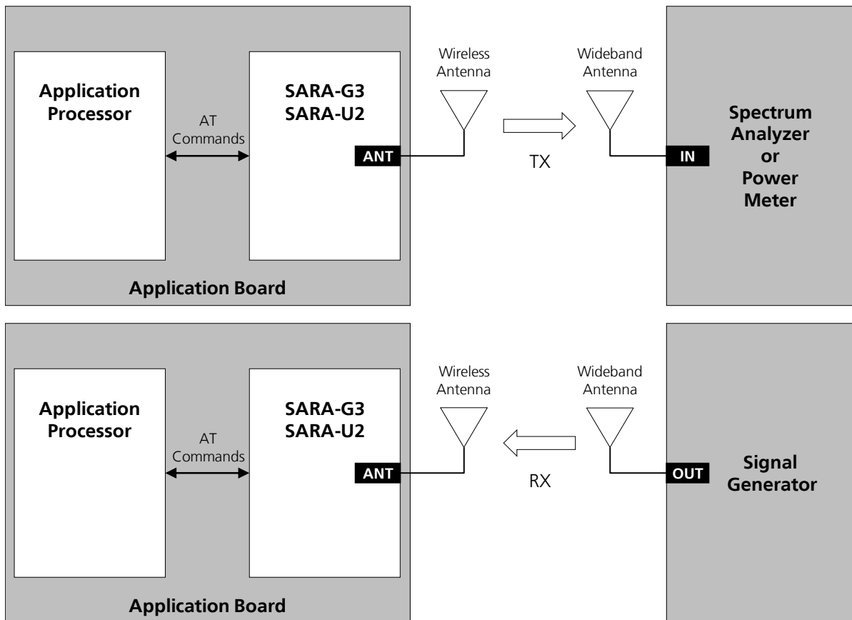
Figure 90: Setup with spectrum analyzer and signal generator for radiated measurement
