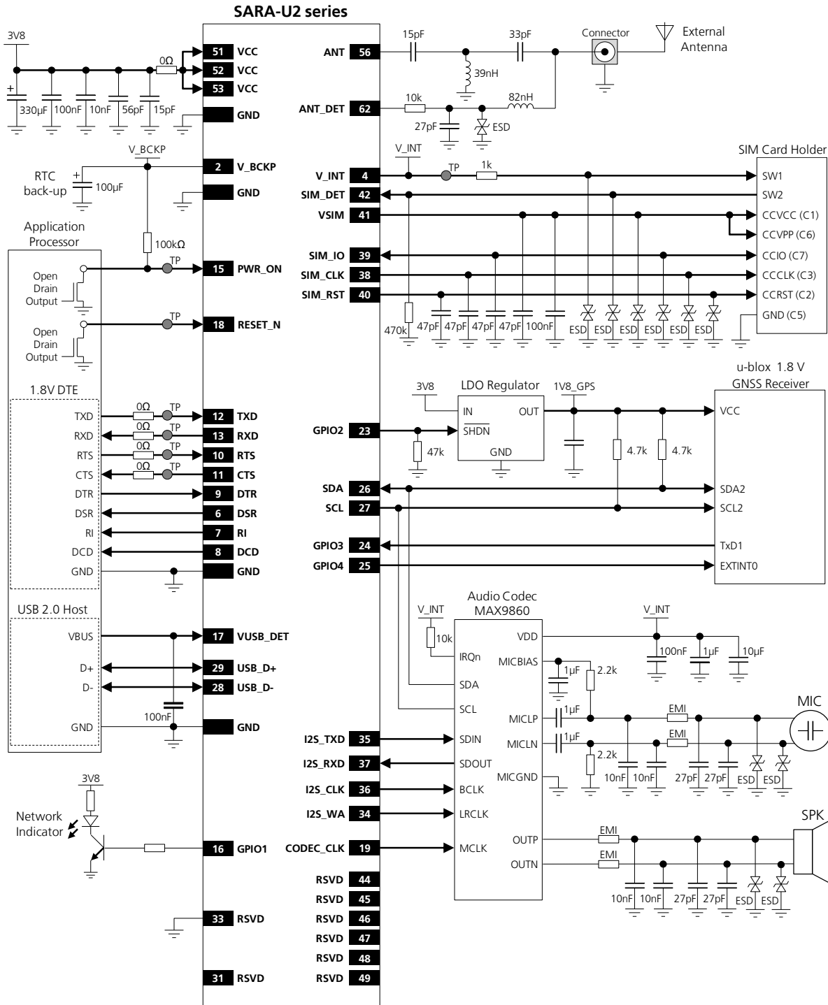
Figure 87: Example of schematic diagram to integrate SARA-U2 module in an application board, using all the interfaces
