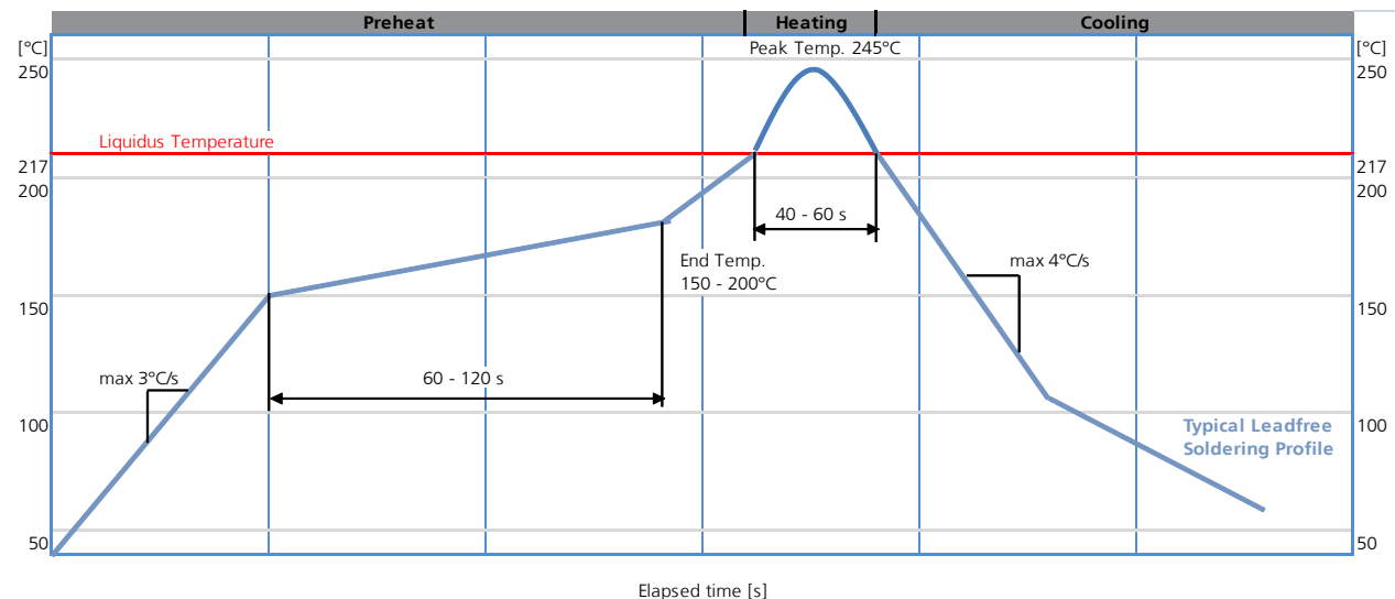
Figure 88: Recommended soldering profile
