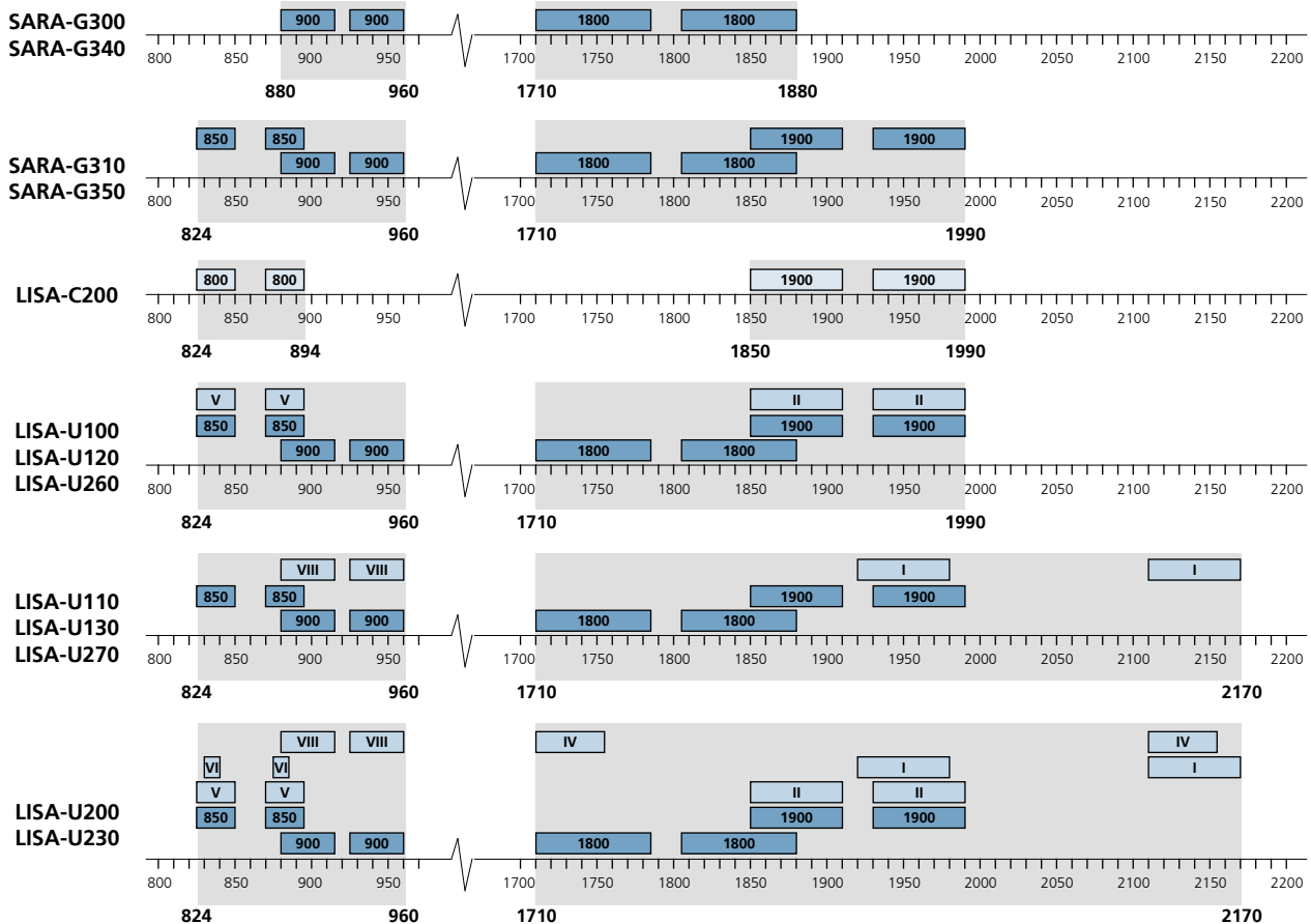
Figure 93: Summary of operating bands frequency ranges among modules
