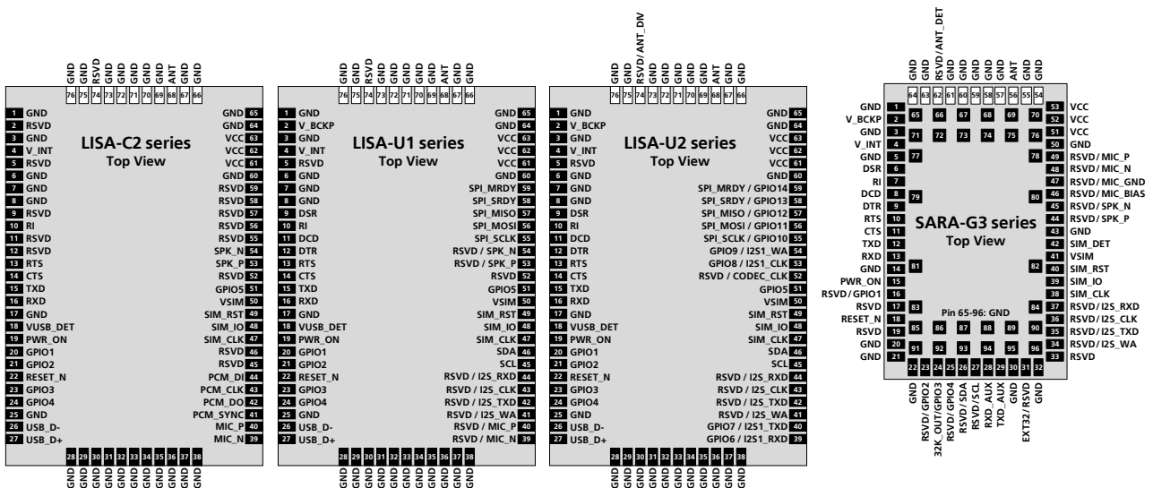
Figure 91: LISA series vs. SARA-G3 series modules pin assignment: highlighted pads that can be shared on the application board
