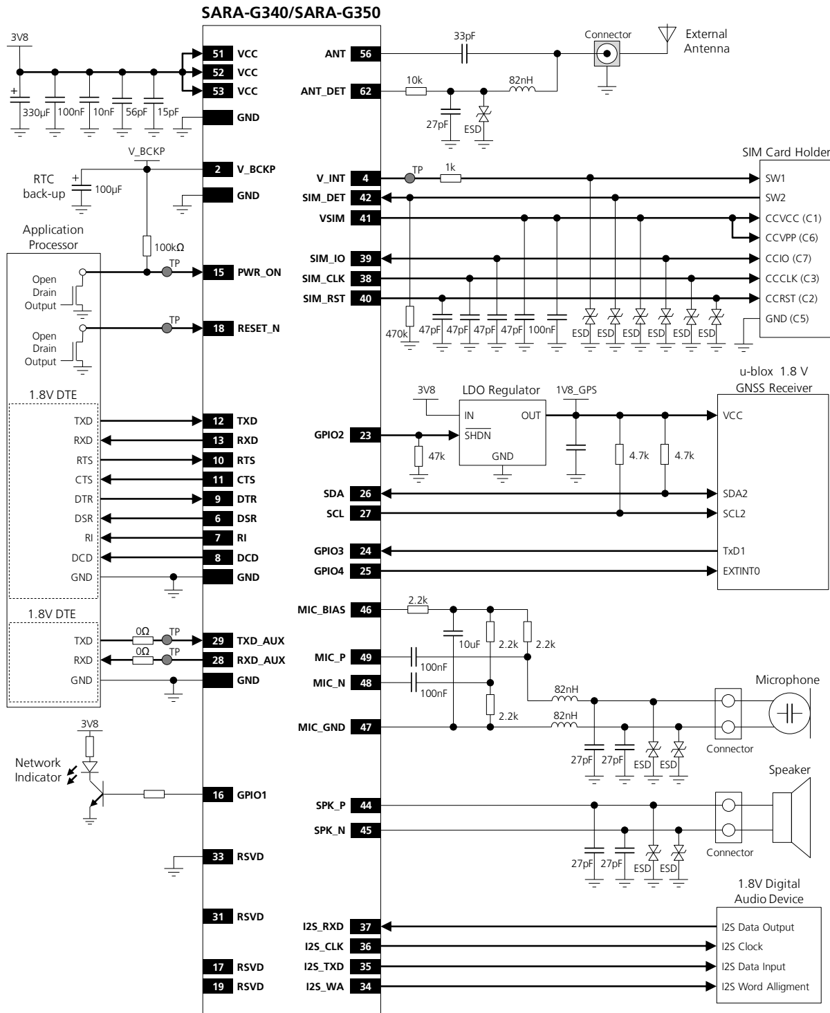
Figure 86: Example of schematic diagram to integrate SARA-G340/G350 module in an application board, using all the interfaces
