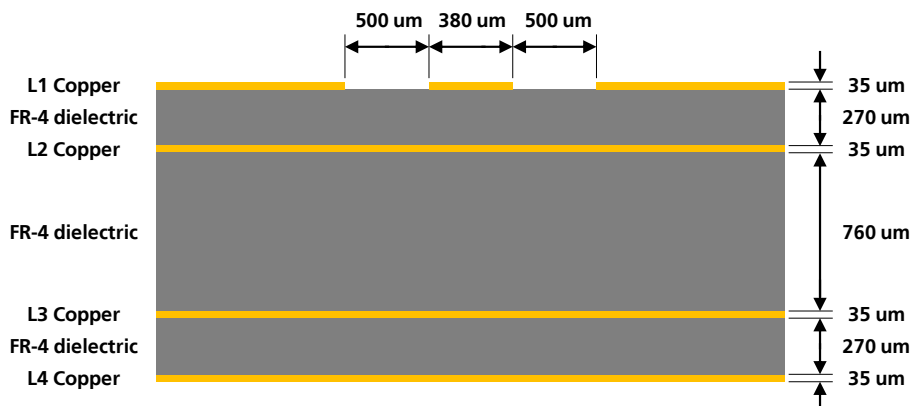
Figure 50: Example of 50 \Omega coplanar waveguide transmission line design for the described 4-layer board layup
