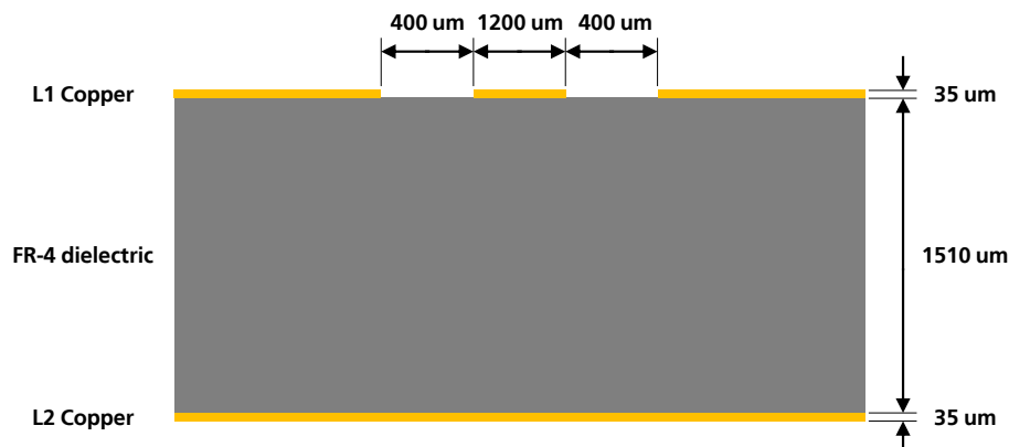
Figure 51: Example of 50 \Omega coplanar waveguide transmission line design for the described 2-layer board layup
