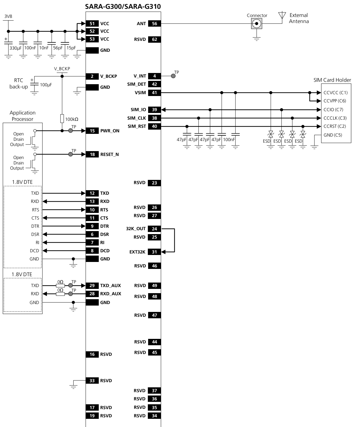
Figure 85: Example of schematic diagram to integrate SARA-G300/G310 modules in an application board, using all the interfaces
