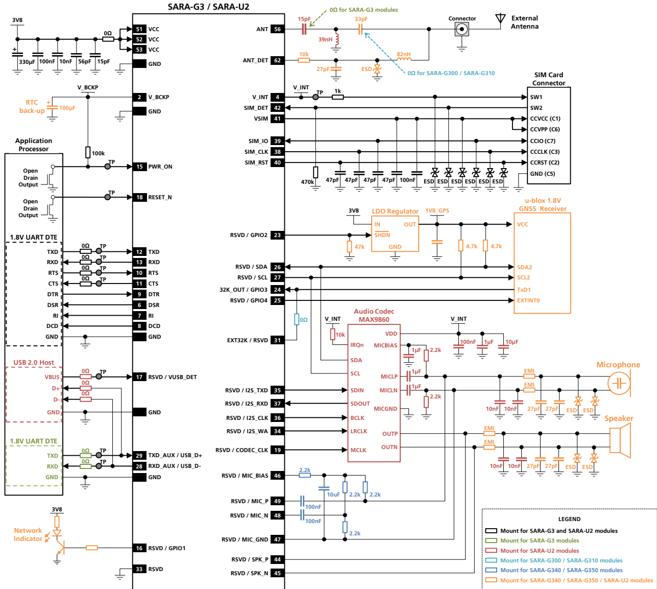
Figure 95: Example of complete schematic diagram to integrate SARA-G3 and SARA-U2 modules on the same application board
