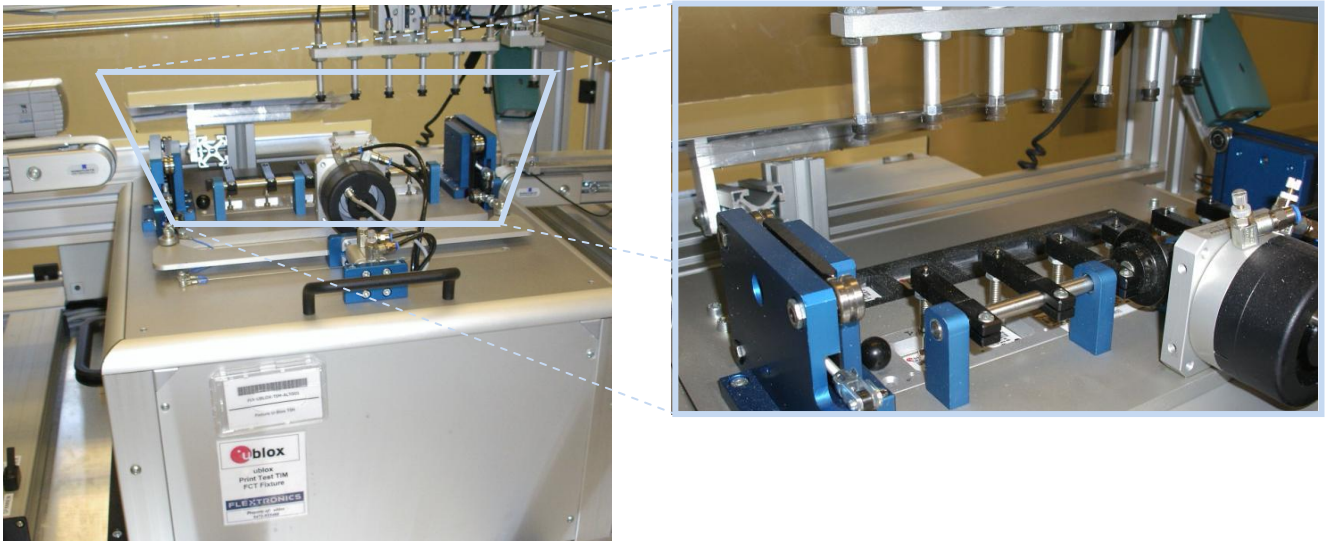
Figure 89: Automatic test equipment for module tests
