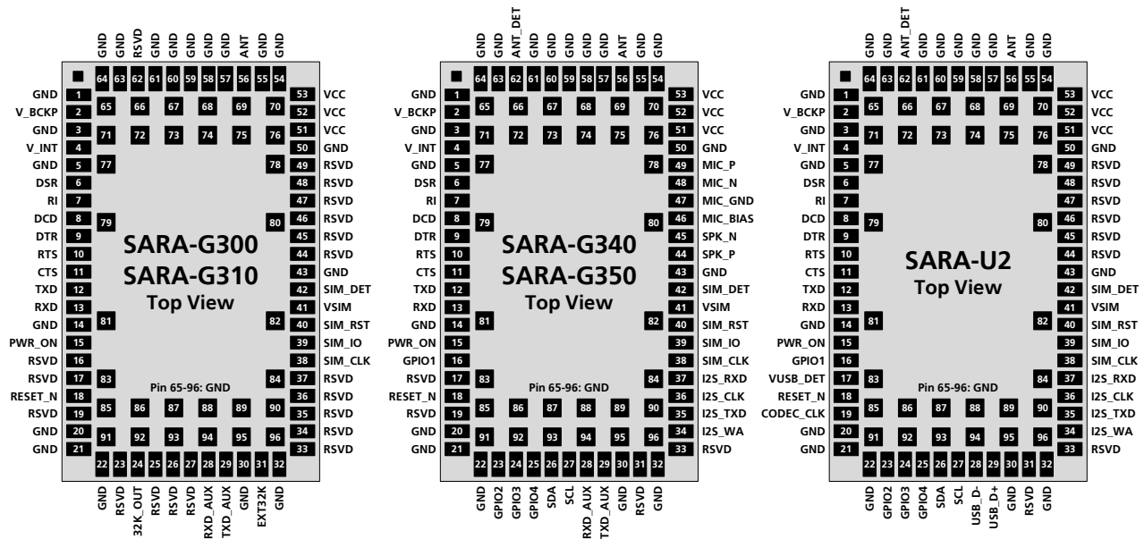
Figure 94: SARA-G3 and SARA-U2 series modules pin layout and pin assignment
