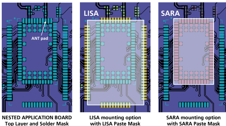
Figure 92: Nested Design concept description: LISA and SARA modules alternatively mounted on the same application board
