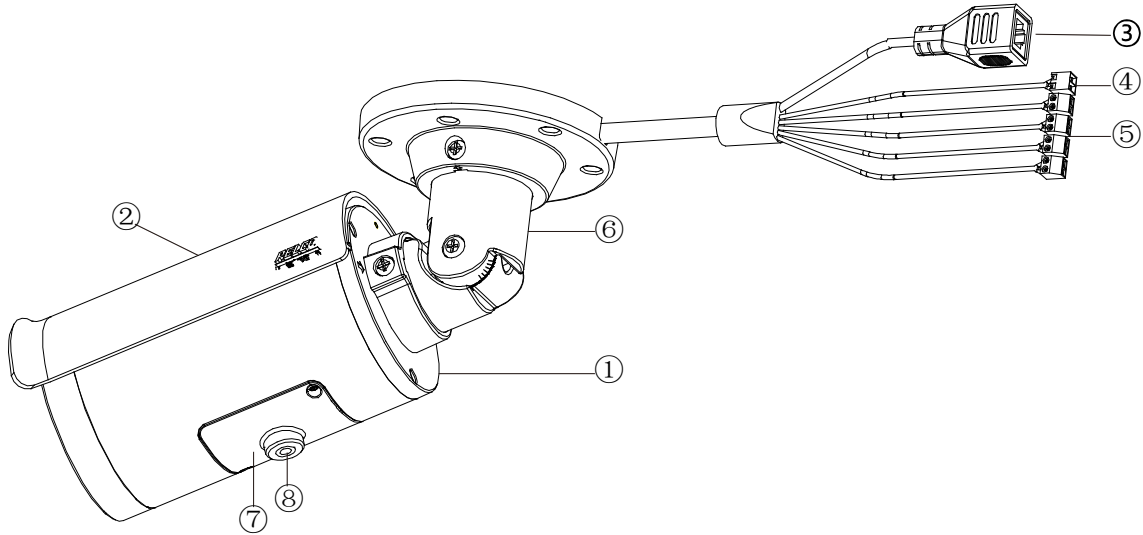
FIGURE 1-2: CAMERA CONNECTIONS AND FEATURES 1/2
