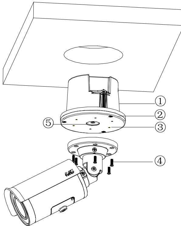
FIGURE 2-4: IN-CEILING INSTALLATION WITH IBPBBAP-EI
