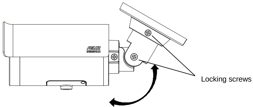
FIGURE 2-5: POSITIONING THE CAMERA 1/2
