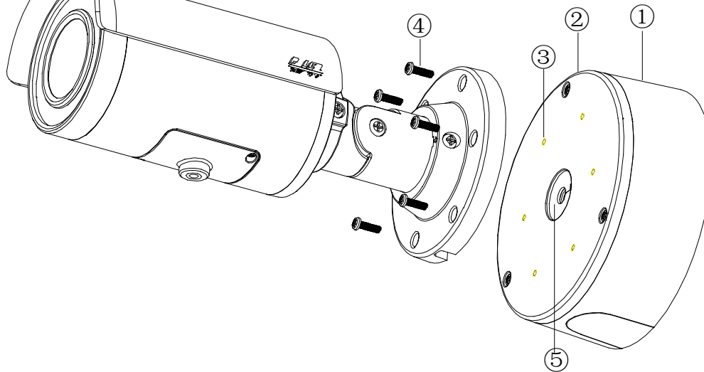
FIGURE 2-3: SURFACE MOUNT WITH IBPBAP-ES
