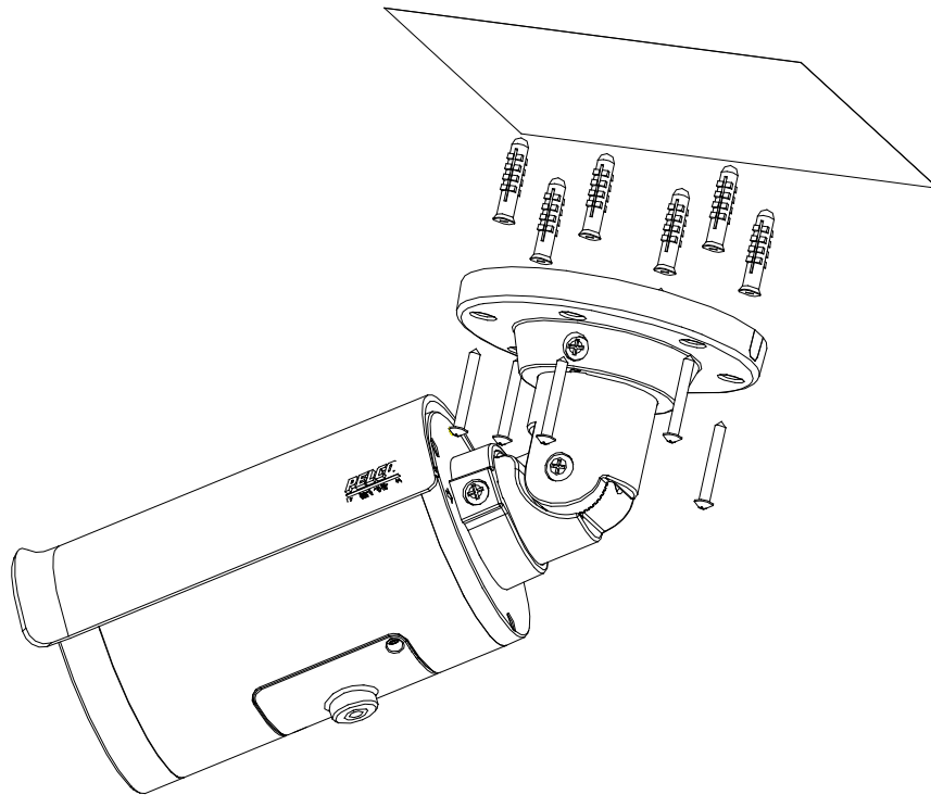
FIGURE 2-1: MOUNTING THE BRACKET
