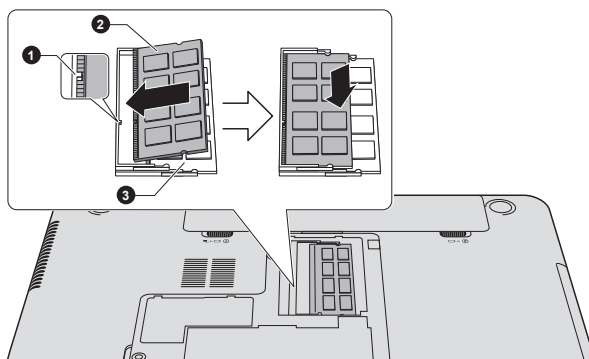
Figure 3-10 Seating the memory module
