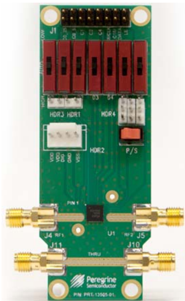
Figure 1. PE43704 Evaluation Board Assembly
