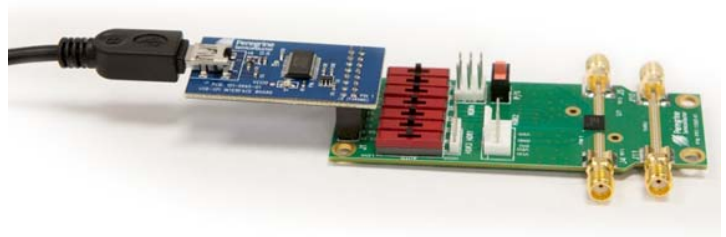
Figure 3. DSA USB Interface Board Connected to the PE43704 Evaluation Board for Latch-Parallel and Serial Programming
