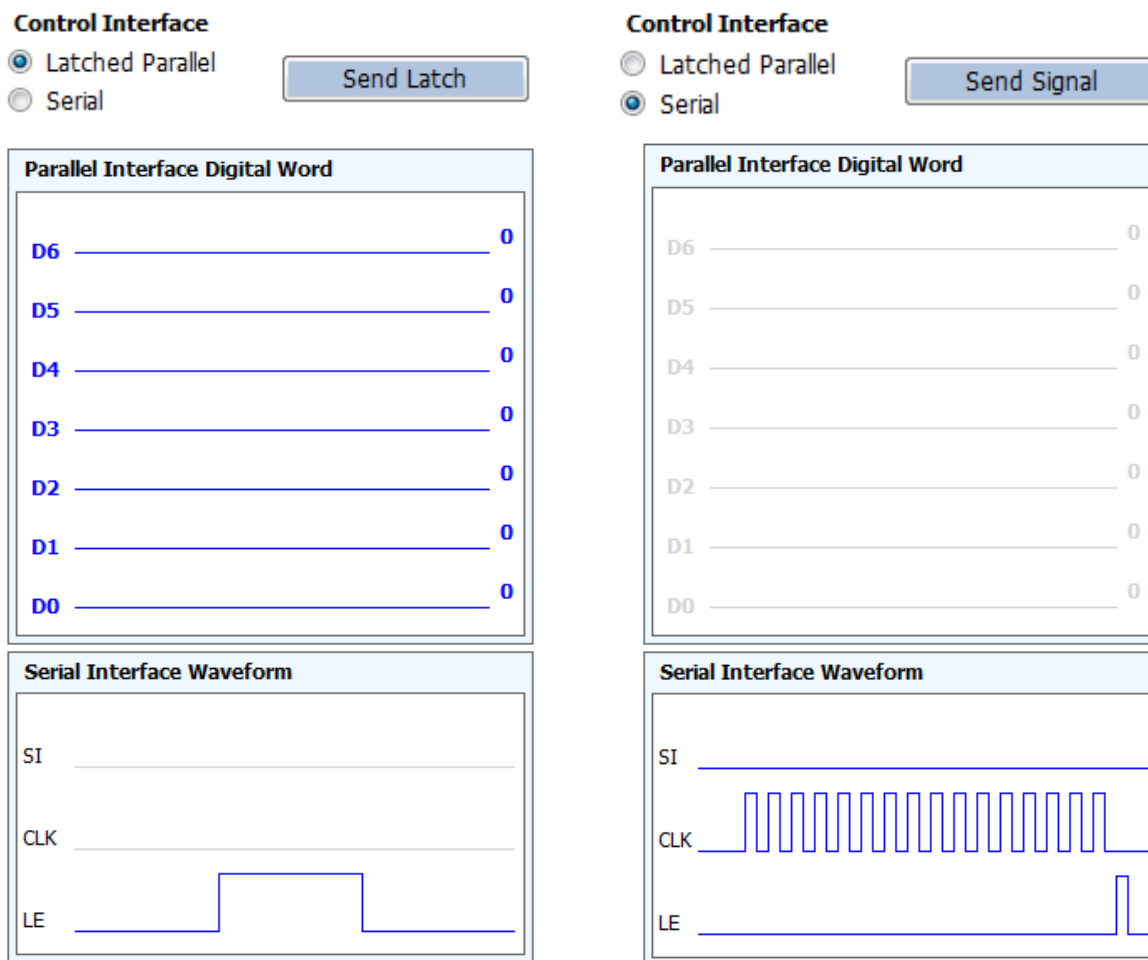
Figure 7. Latched-Parallel or Serial Mode
