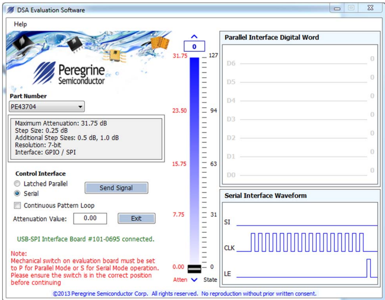
Figure 6. DSA Application Software Graphical User Interface (GUI)
