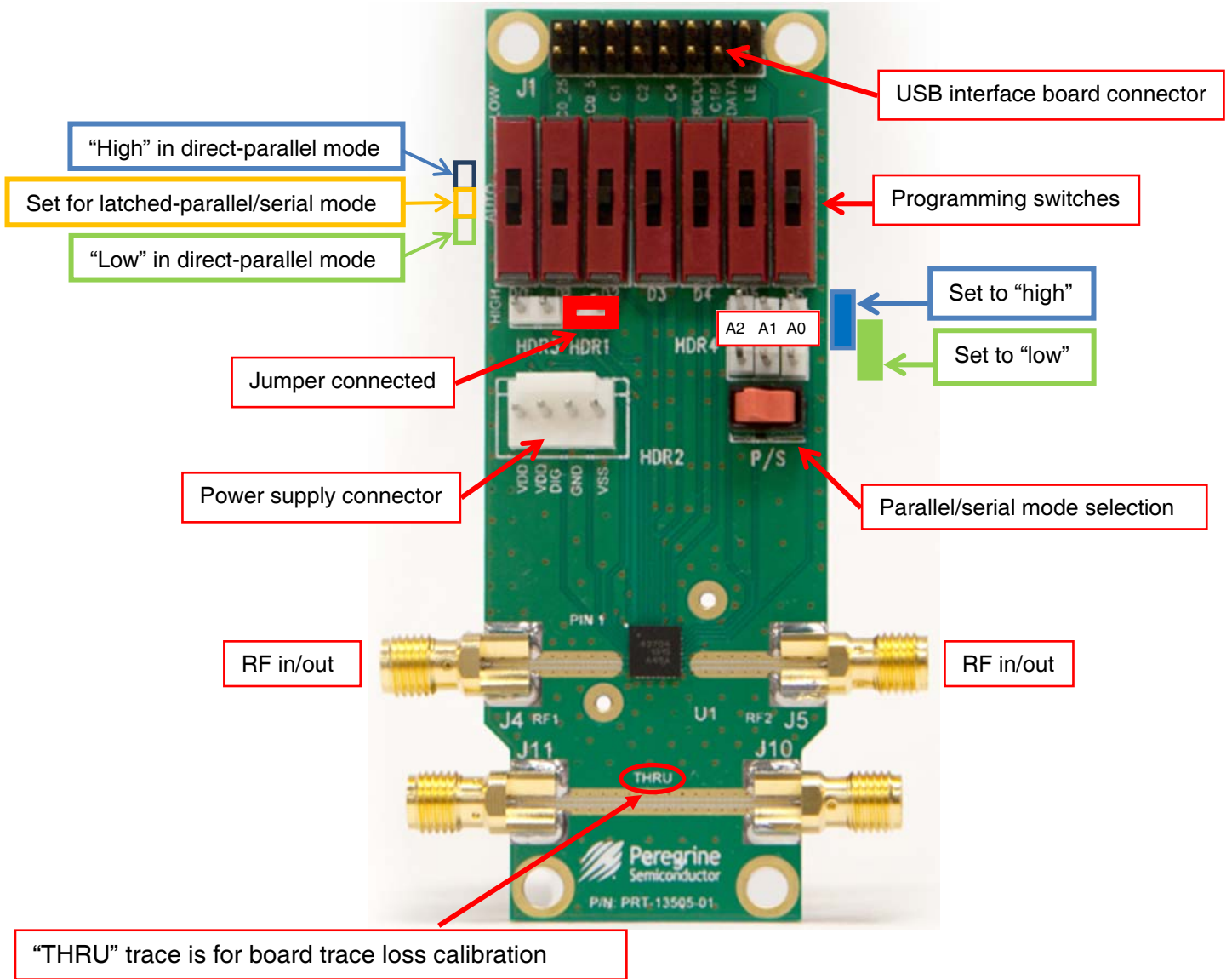
Figure 9. PE43704 Evaluation Board Outline Showing Functional Overview
