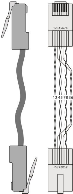
Figure 8: TP PINOUT
