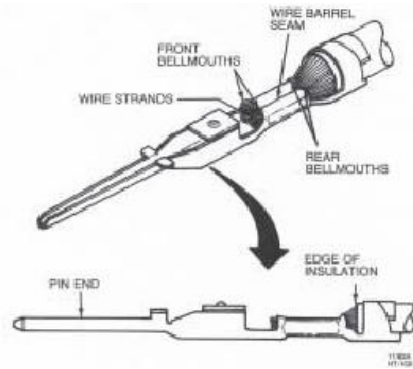
Figure 4. Correctly Crimped Terminal
