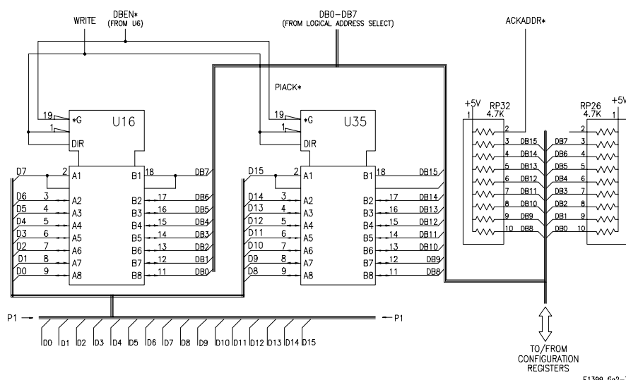
Figure 2-7. Data Bus Drivers
