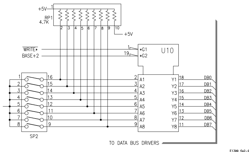
Figure 2-9. Device Type Register
