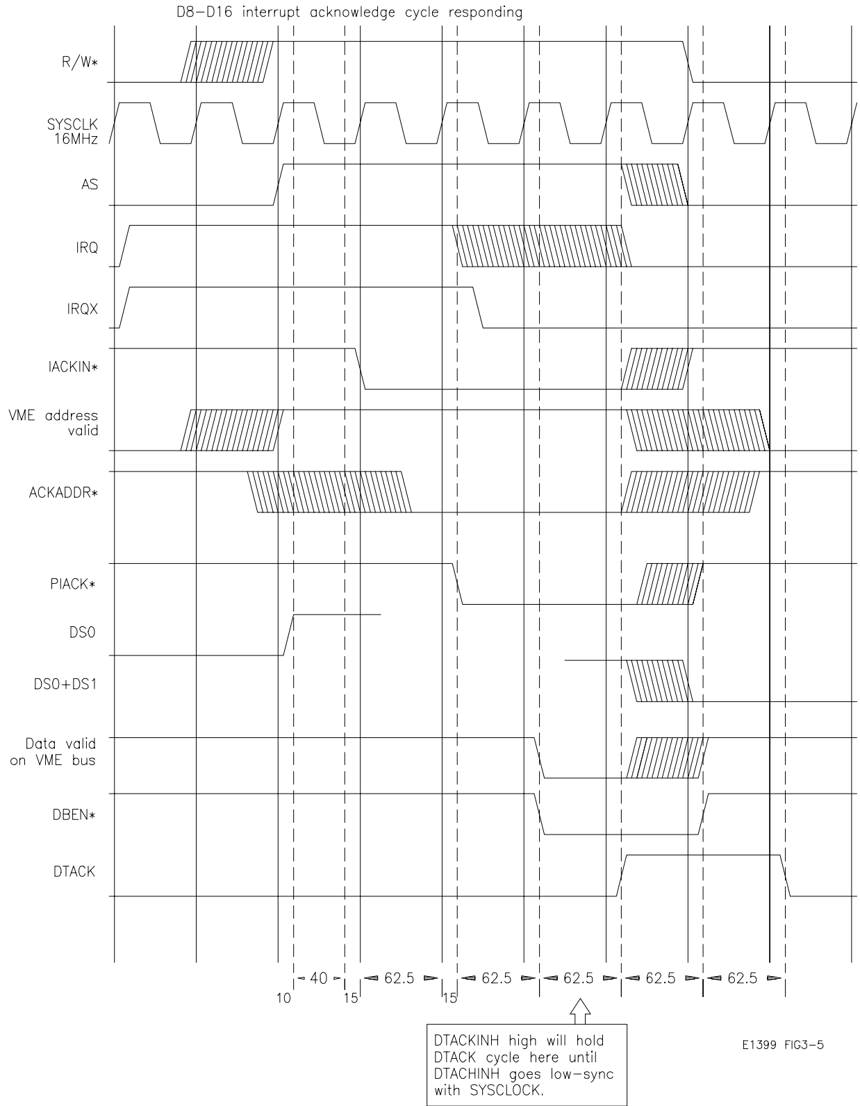
Figure 3-5. Interrupt Timing
