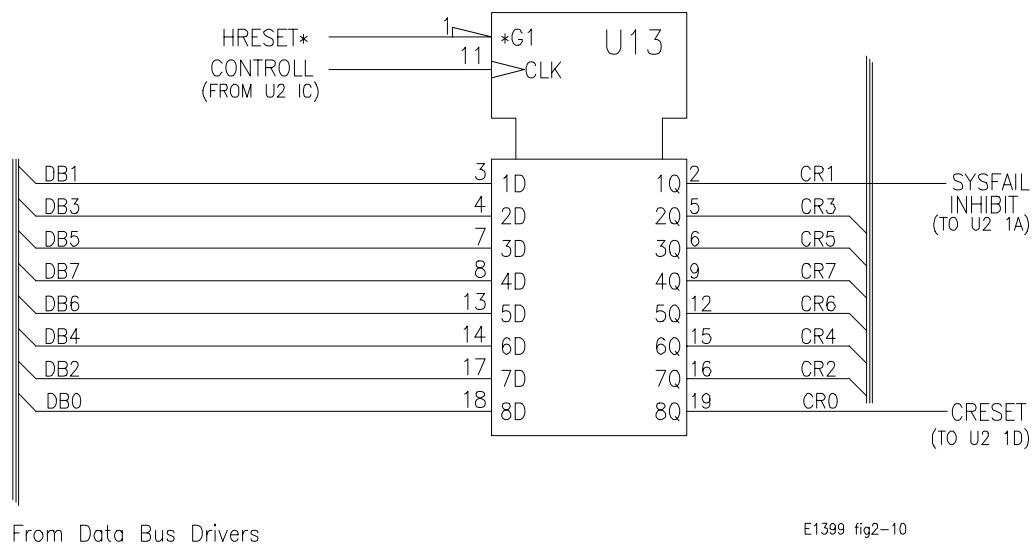
Figure 2-10. Control Register
