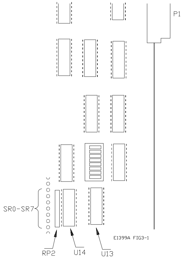
Figure 3-1. Status Register Access Points
