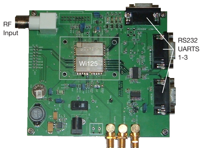
Figure 1 Wi125 Evaluation Board
