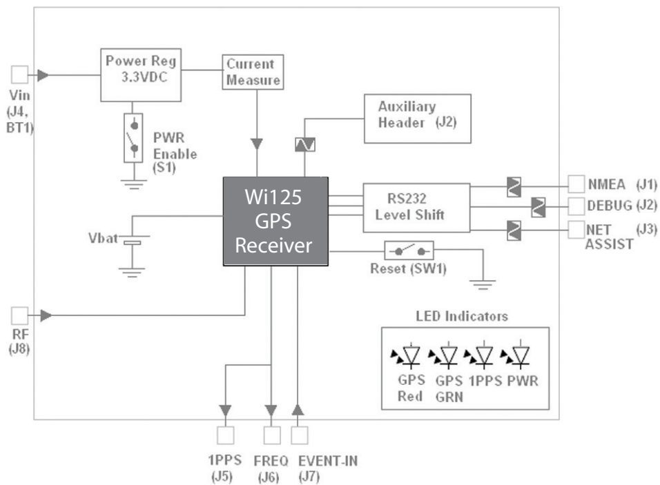
Figure 2 Wi125 Block Diagram
