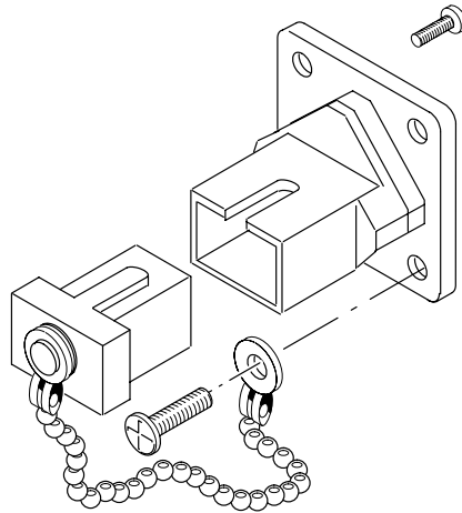
Figure F-5: SC Optical Bulkhead Assembly
