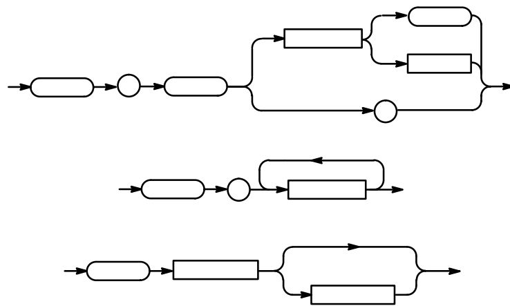
Figure 3-3: Typical Syntax Diagrams
