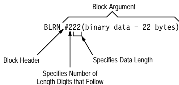
Figure 3-2: Block Argument Example
