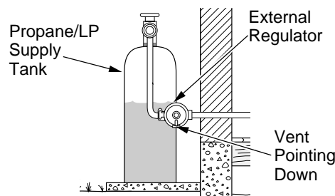
Figure 12 - External Regulator With Vent Pointing Down
