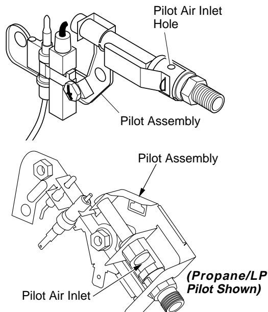
Figure 22 - Pilot Inlet Air Hole
