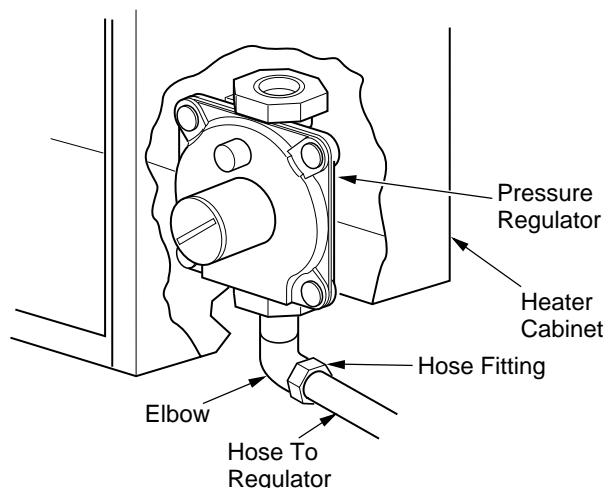
Figure 11 - Gas Connection
