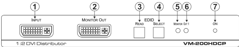
Figure 1: VM-200HDCP 1:2 DVI Distributor Front Panel
