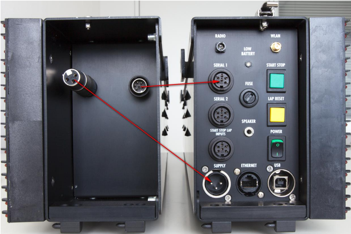
Figure 5 - Cable connection
