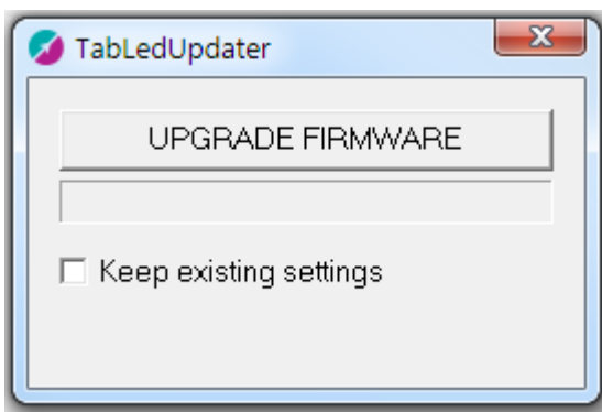
Figure 11 – Updater Software
