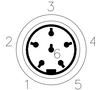
Figure 4 - 6-pole Amphenol connector
