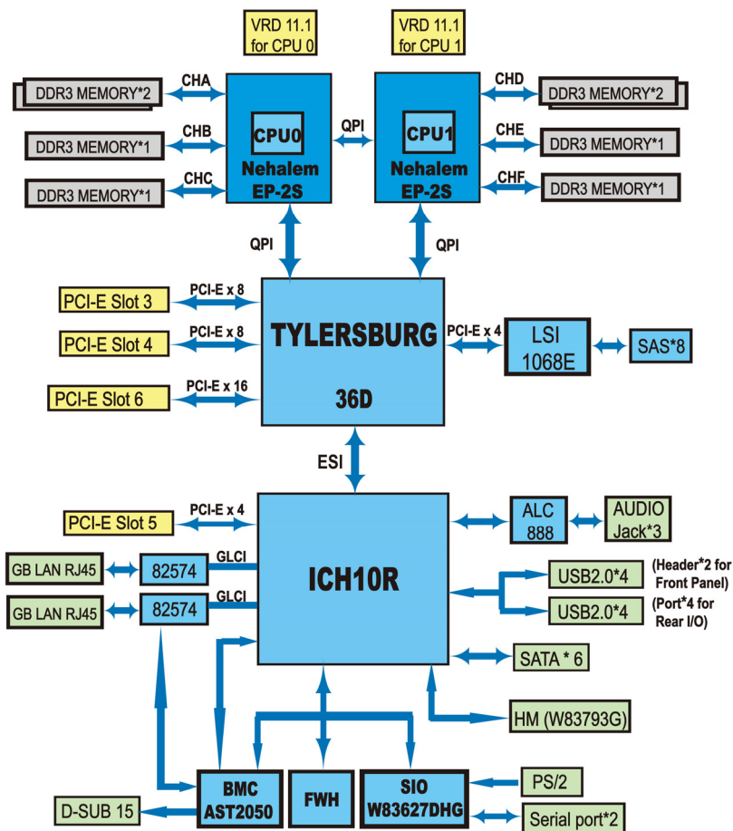
S7002 Block Diagram (Represents all SKUs)
