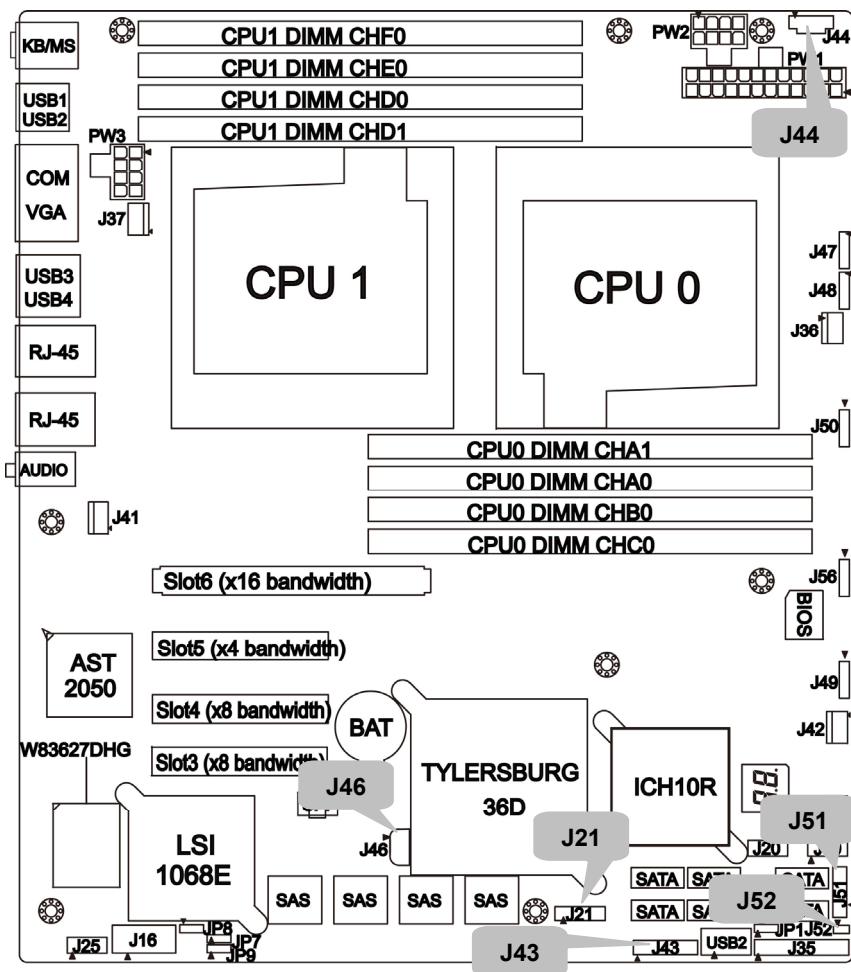
J21/J51 SAS SGPIO Header
