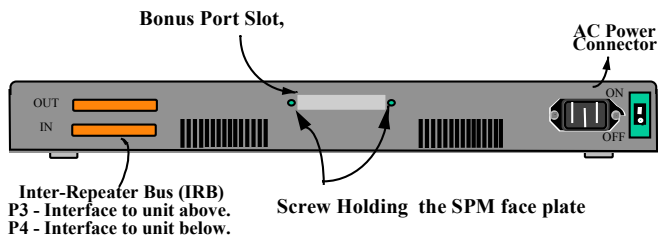
Figure 3.10c: Rear View - SPM Retaining Screws in Face Plates
