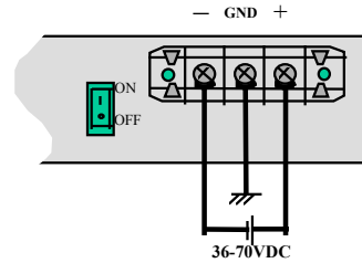
Figure B4.1: -48VDC Terminal Block on Magnum 8000X -48VDC
