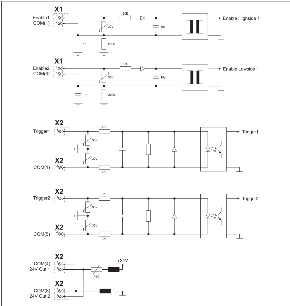
Figure 113: Input/output circuit diagram 8BVI0014HxS0.000-1, 8BVI0028HxS0.000-1, 8BVI0055HxS0.000-1, 8BVI0110HxS0.000-1
