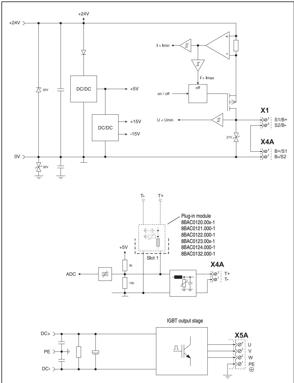
Figure 113: Input/output circuit diagram 8BVI0014HxS0.000-1, 8BVI0028HxS0.000-1, 8BVI0055HxS0.000-1, 8BVI0110HxS0.000-1 (Forts.)
