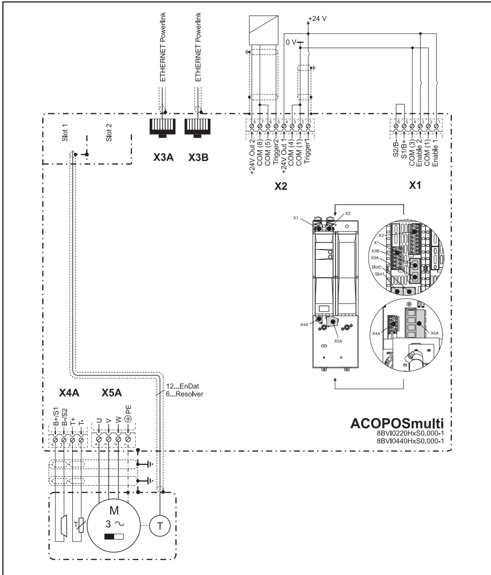
Figure 110: Overview of pin assignments - 8BVI0220HxS0.000-1, 8BVI0440HxS0.000-1
