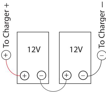
12 VOLT (Series Connected) = 24V
