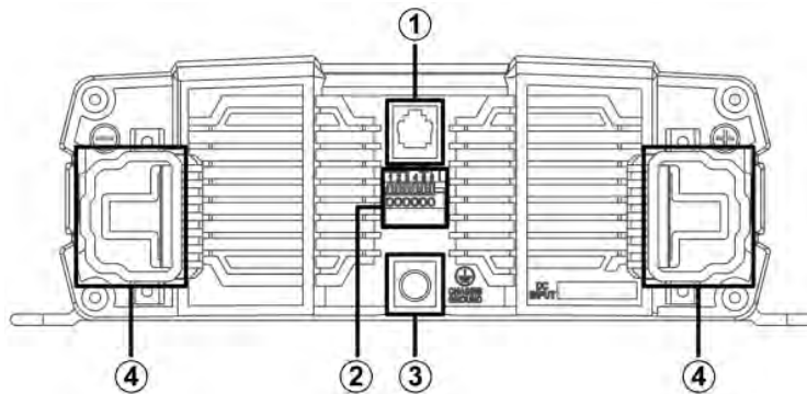
Figure 11. SP-1500/2000
