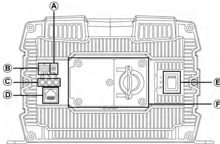
Figure 7. SP-3000/4000 AC output panel view
