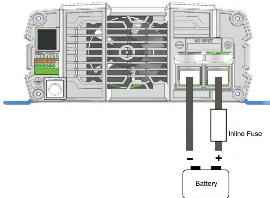
Figure 16. Battery cabling
