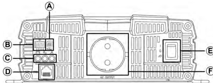
Figure 6. SP-1500/2000 AC output panel view
