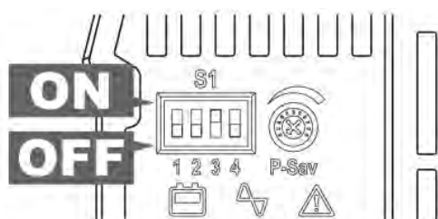
Figure 8. DIP switch ON/OFF position
