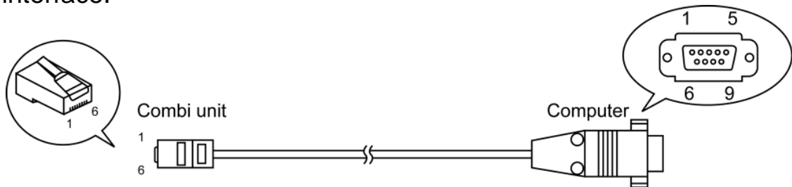
Figure 17. RS232 cable
