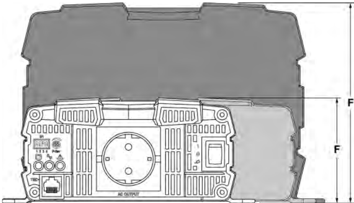
Figure 4. SP series drawing (AC output/Front View)
