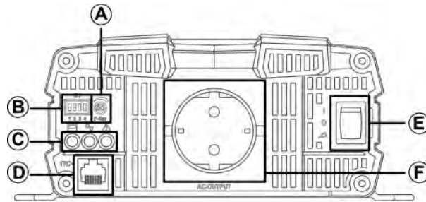
Figure 5. SP-700/1000 AC output panel view
