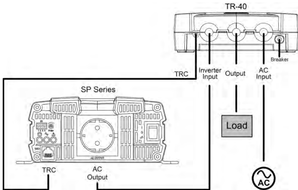
Figure 9. Wiring between SP series and TR-40
