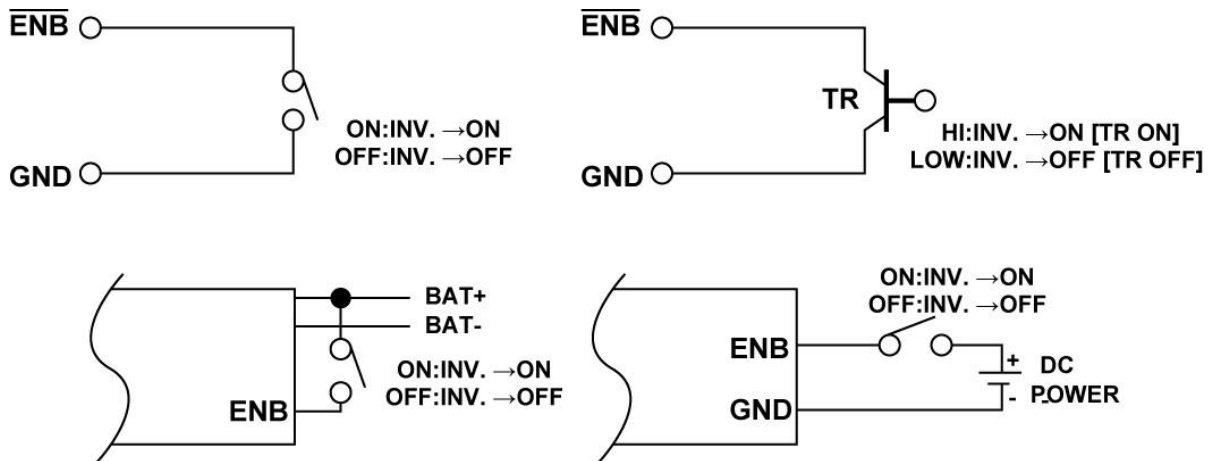
Figure 14. Wiring for control
