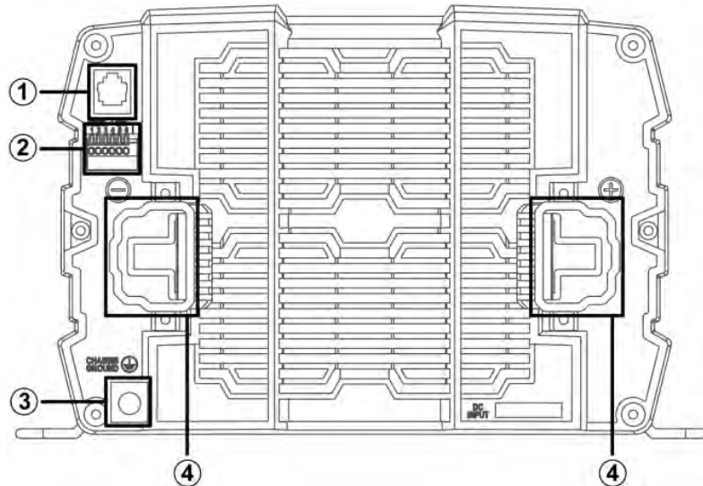
Figure 12. SP-3000/4000
