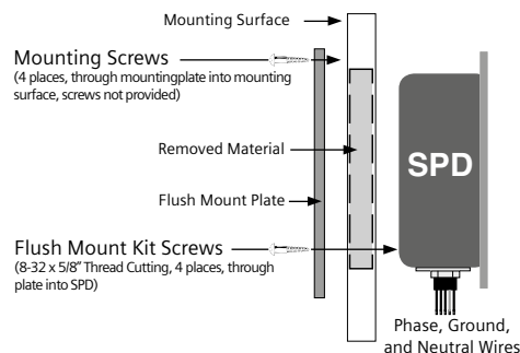
Figure 4: Typical Flush Mount Installation
