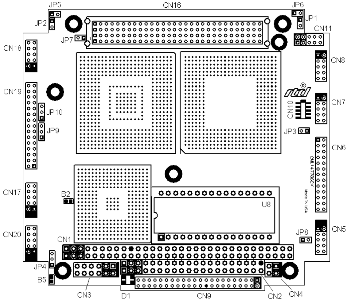
Figure 3: CML147786CX Connector Locations
