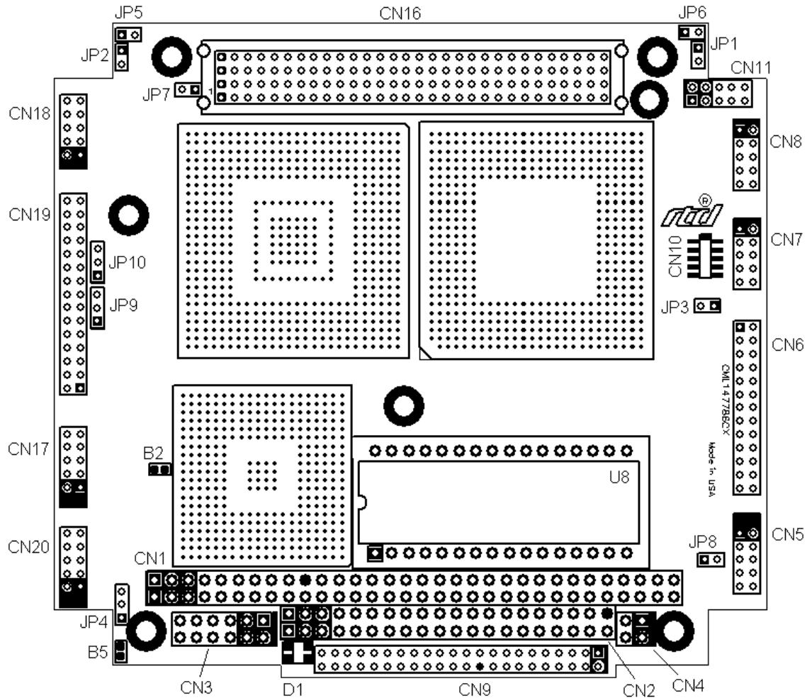
Figure 2: CML147786CX Basic Connector Locations
