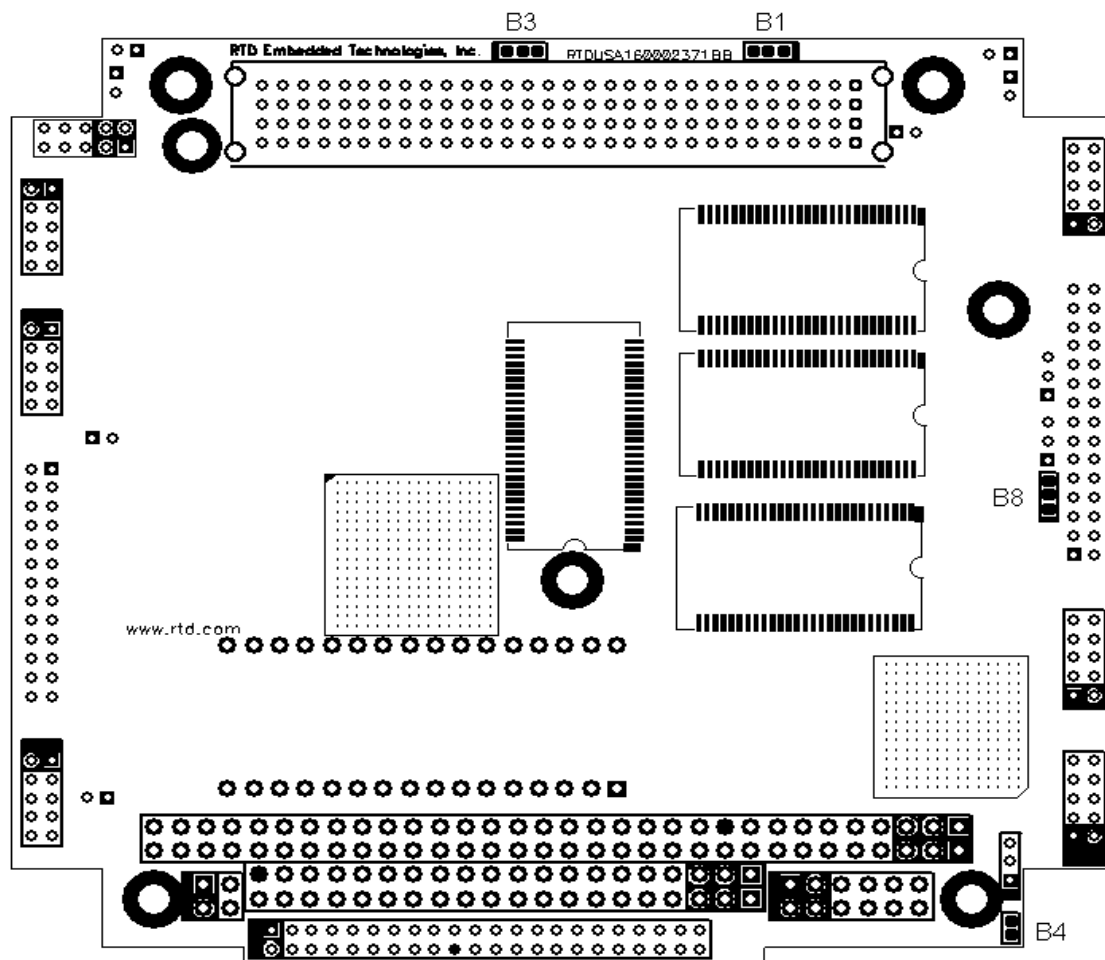
Figure 5: CML147786CX Jumper Locations - Bottom
