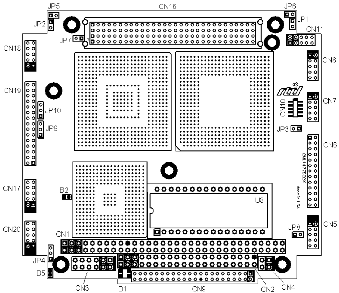
Figure 4: CML147786CX Jumper Locations - Top
