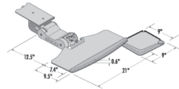
Model C-24-S
