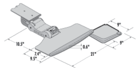
Model LT-24-S
