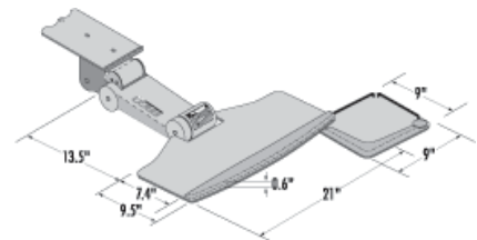
Model T-24-S
