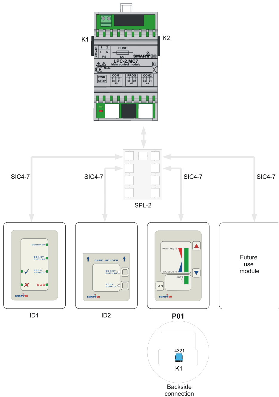
Figure 2: Connection scheme
