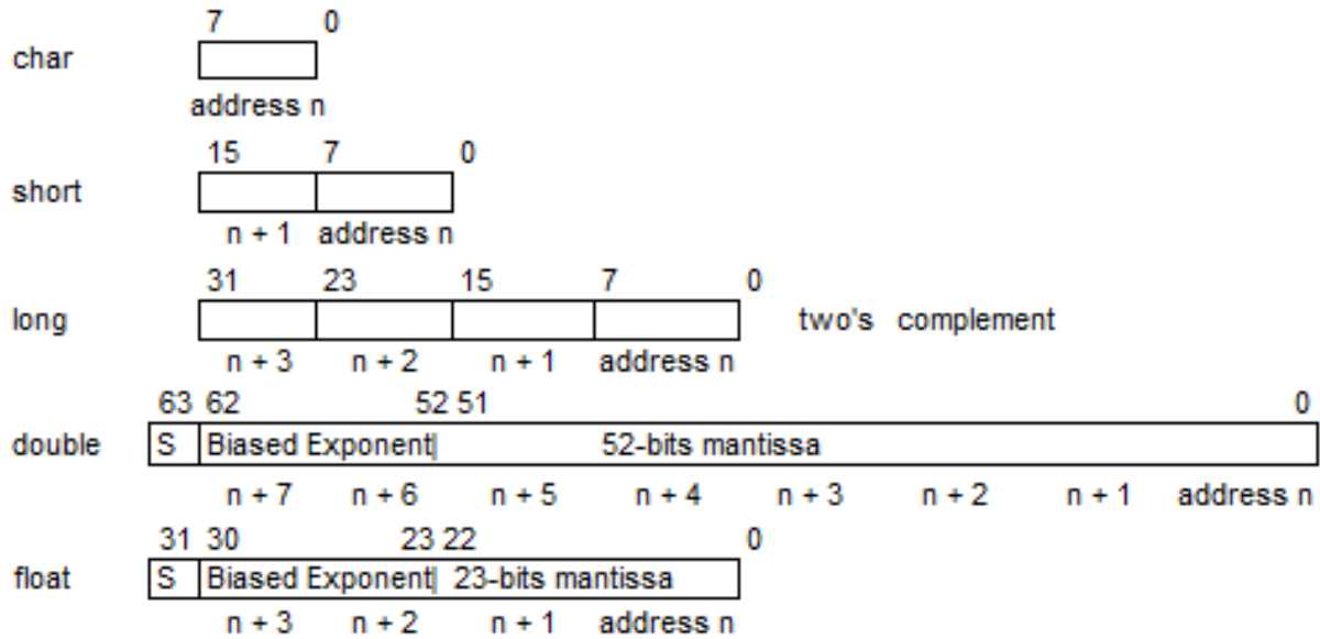
Figure 1: Byte Arrangements
