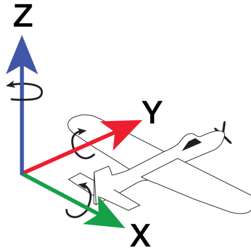
Figure 6: Vehicle Frame
