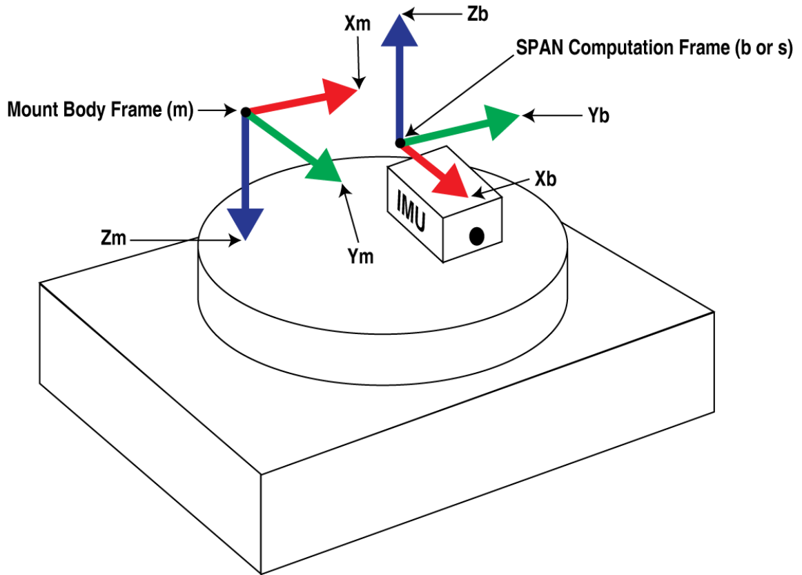
Figure 4: Simple Configuration
