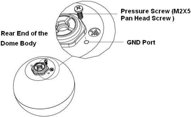
Figure 3-3 Device installation illustration 3
