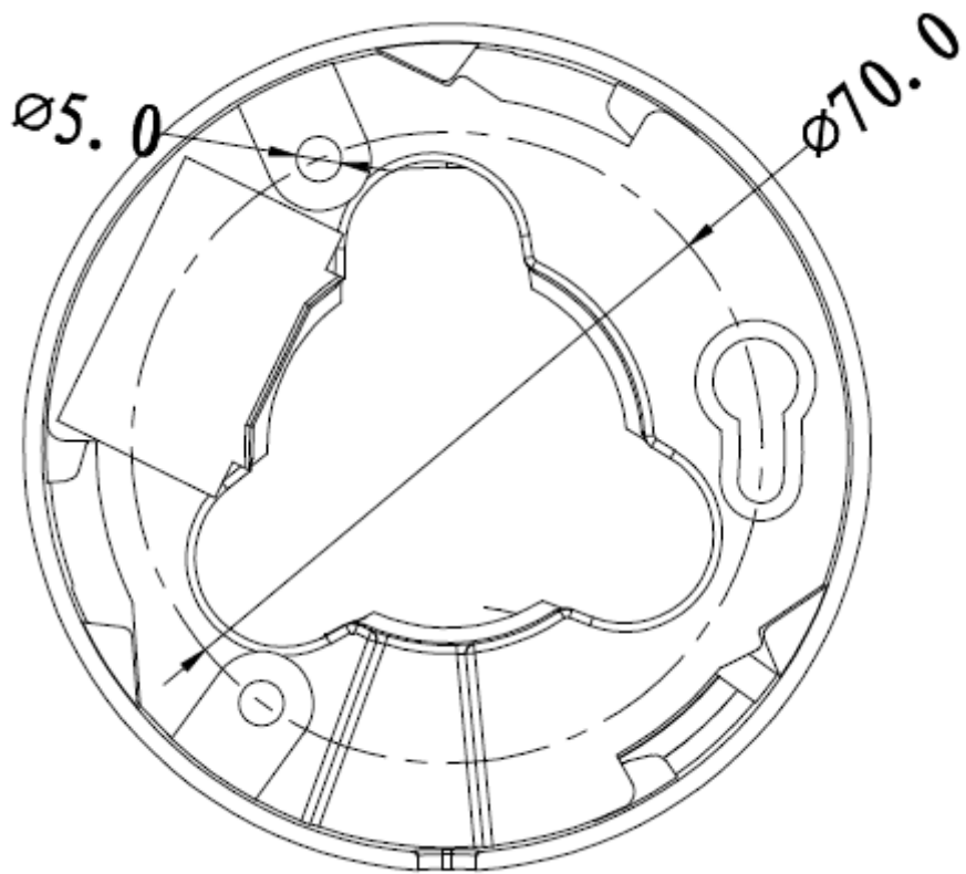
Figure 2-3 Dimension illustration 2
