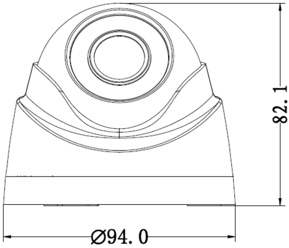
Figure 2-2 Dimension illustration 1
