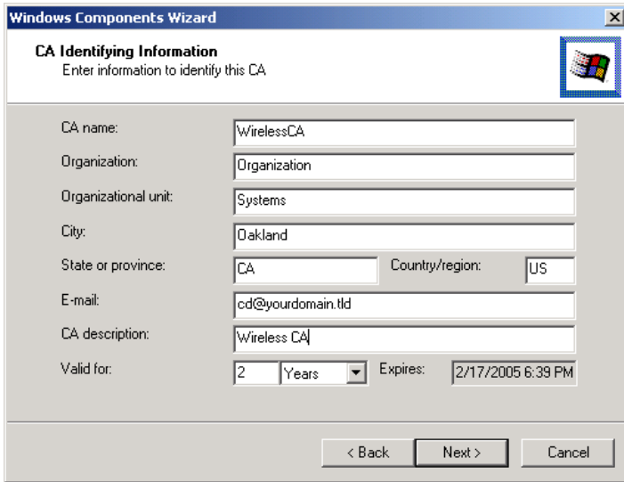
Figure 35: CA Screen
