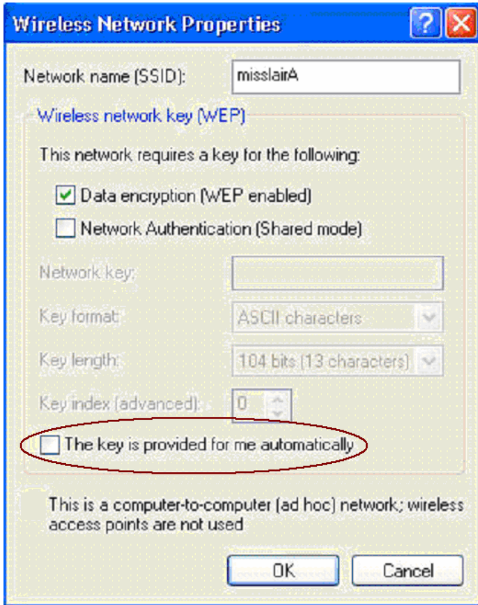
Figure 58: Properties Screen
