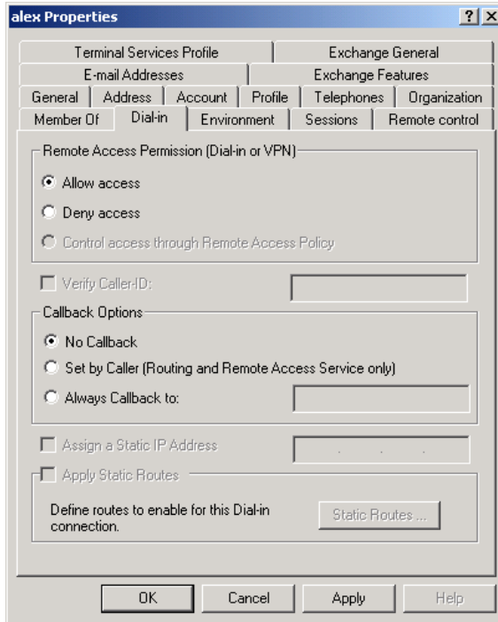
Figure 48: Dial-in Screen
