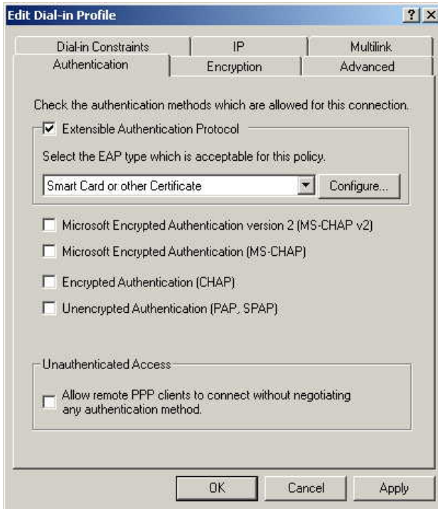
Figure 47: Authentication Screen
