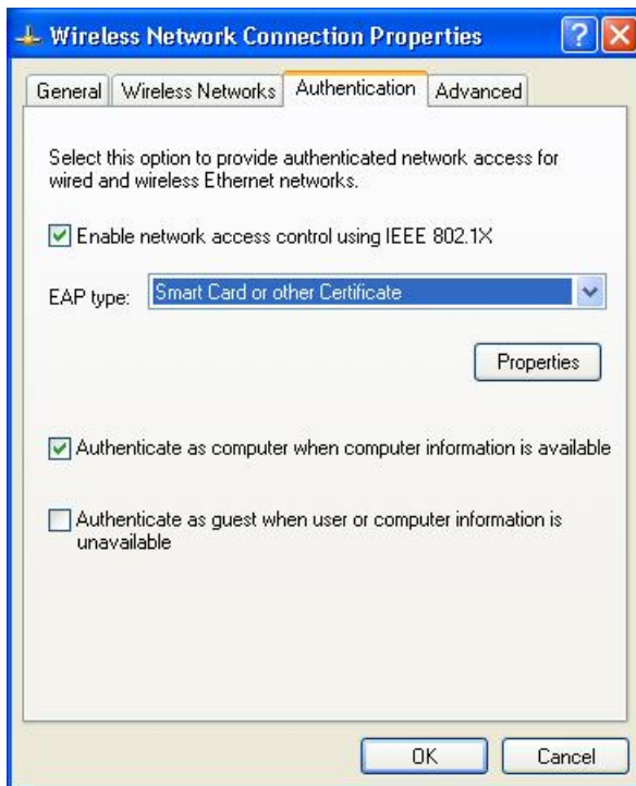
Figure 55: Authentication Tab
