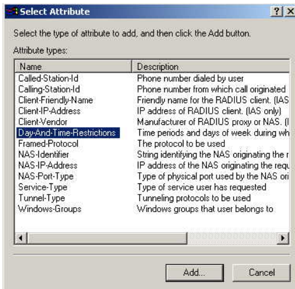
Figure 46: Attribute Screen
