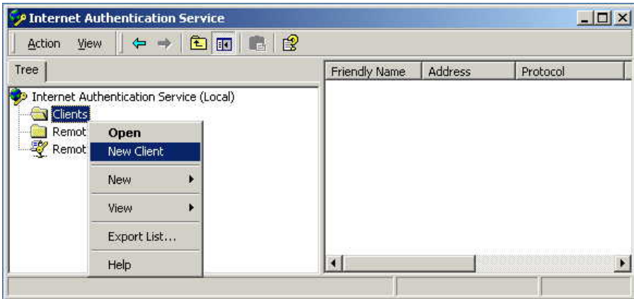
Figure 45: Service Screen
