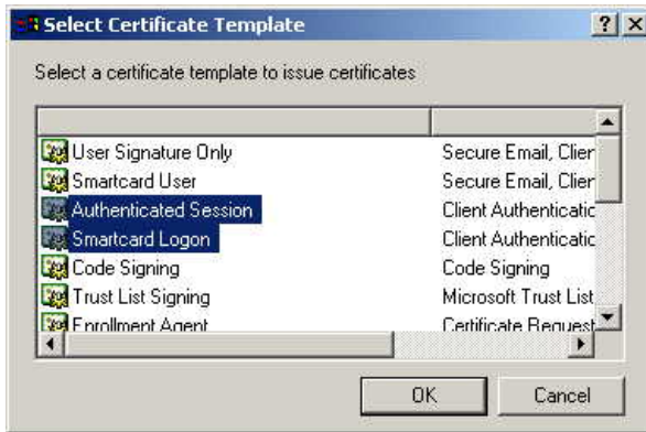
Figure 40: Template Screen
