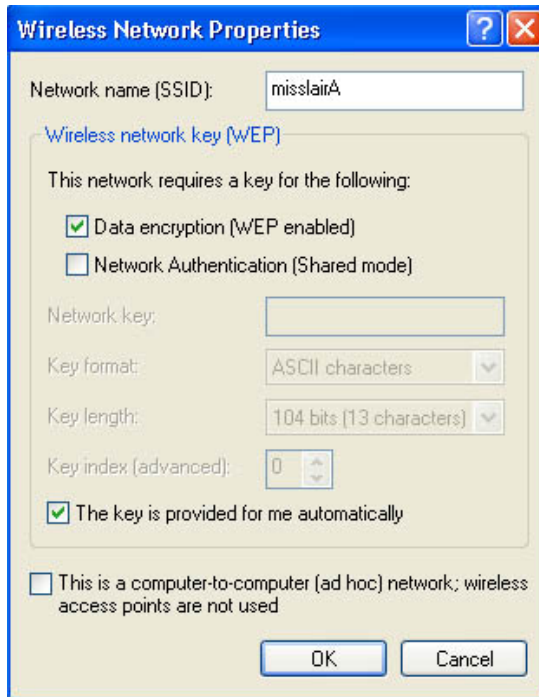
Figure 57: Properties Screen
