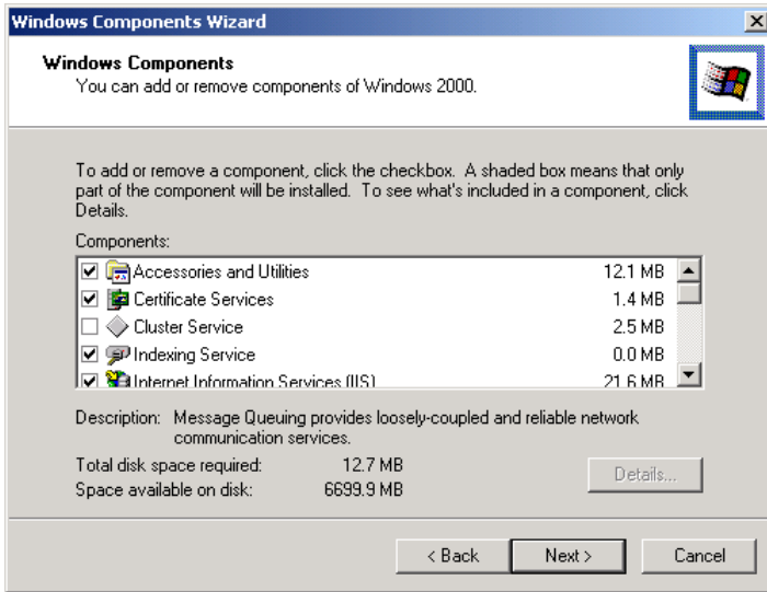
Figure 33: Components Screen
