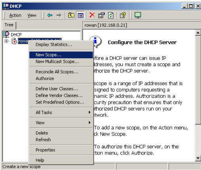
Figure 36: DHCP Screen
