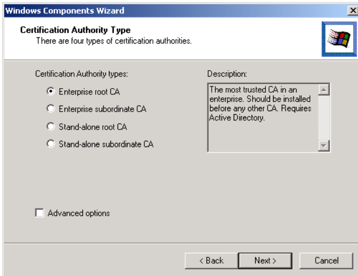
Figure 34: Certification Screen
