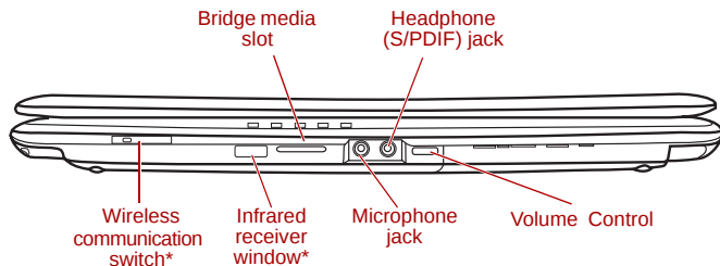
Figure 2-1 Front of the computer with display closed
