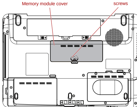
Figure 8-5 Seating the memory module cover
