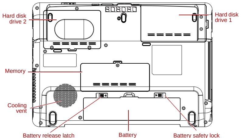
Figure 2-5 The underside of the computer
