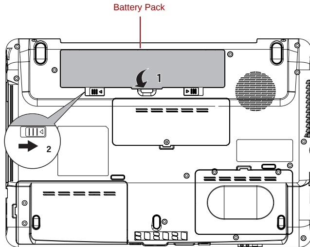
Figure 6-3 Securing the battery pack
