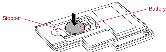
Figure 2-13 Inserting the battery
