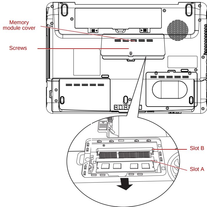
Figure 8-4 Removing the memory module cover
