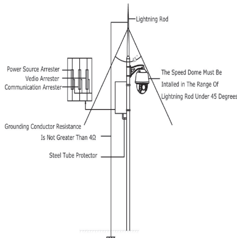
Figure 6.1 Installation Diagram
