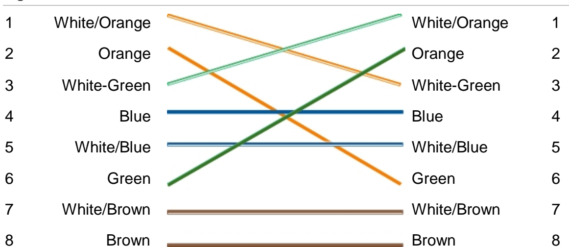
Figure 22: Cross-over cable
