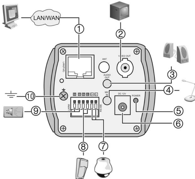
Figure 3: Wiring the camera
