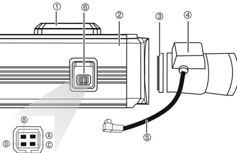
Figure 2: Side elevation of the camera
