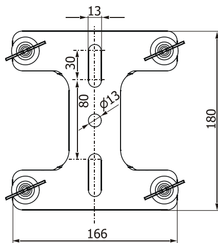
Mounting adapter for one Omega holder
