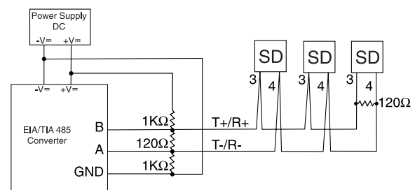
Figure 17c — Wiring bias and termination resistors. Controllers must be wired in a daisy chain configuration.
