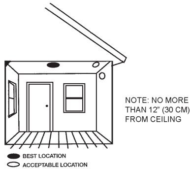
FIGURE 5: RECOMMENDED SMOKE ALARM MOUNTING LOCATION
