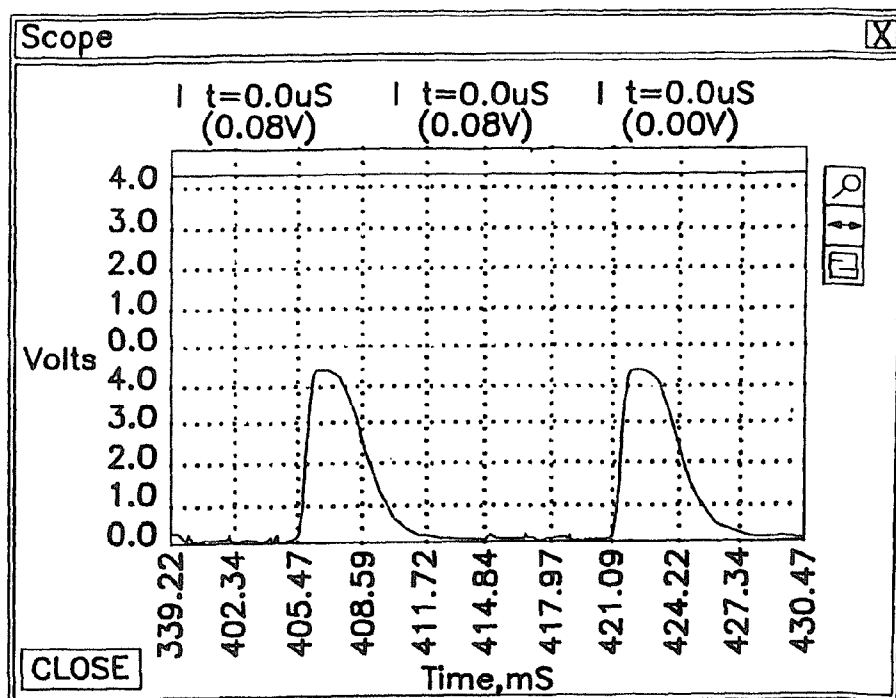
CRT photoresponse
