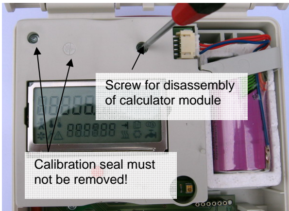
Picture 3: calculator housing 2: removal of calculator module
