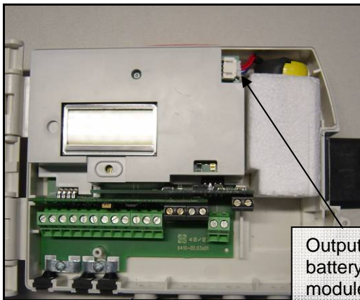
Picture 5: inside view with battery calculator housing 1
