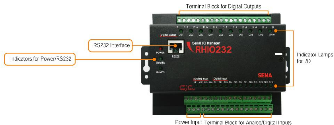
Figure 2-1. The panel layout of the Rhio232
