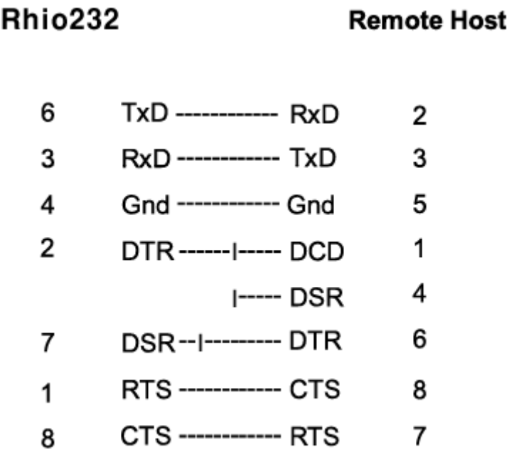
Figure A-5. RS232 serial port wiring diagram
