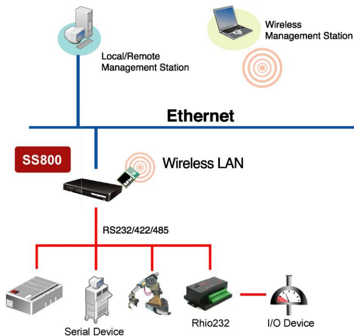
Figure 5-1 Application diagram of the Rhio232 and the SS800
