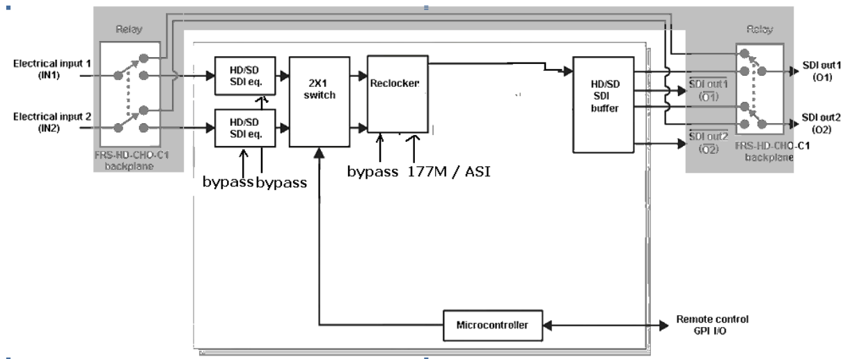
Figure 1: HDSDI-CHO-2x1(-PB) functional overview
