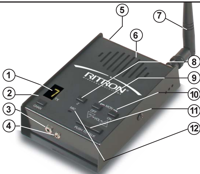
FIG-1: RADIO CONTROLS & CONNECTORS
