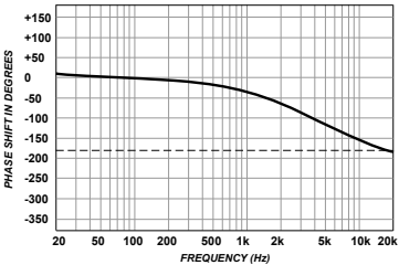
At this setting 200Hz is shifted by just one or two degrees while 20kHz is shifted 180°.
