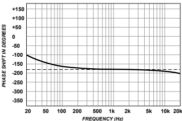
Near maximum setting 200Hz reaches 180°.
