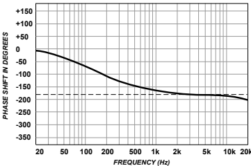
At this setting 200Hz is shifted by 100° while everything above 2kHz is shifted 180°.
