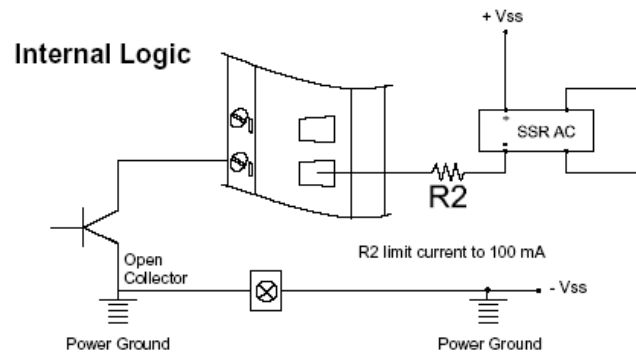
Figure 42: Digital output used with SSR (ADAM-5050/5056)
