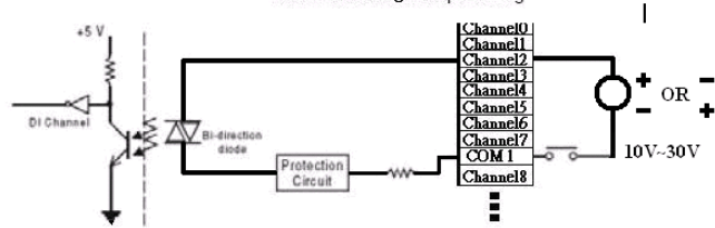
ADAM-5038S Digital Input Wiring
