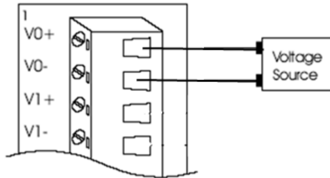
Figure 22: Applying calibration voltage
