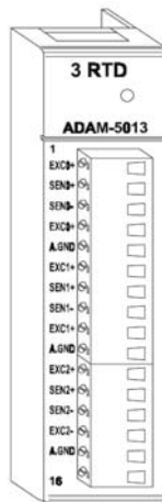
Figure 1: ADAM-5013 module frontal view
