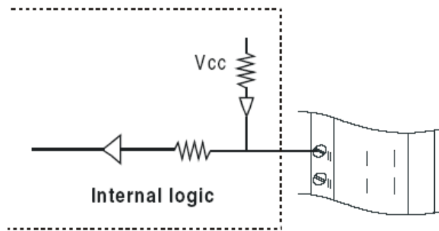
Figure 54: TTL Input Level
