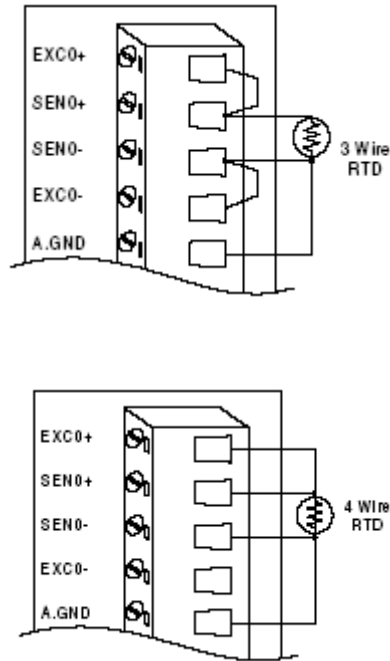
Figure 2: RTD inputs
