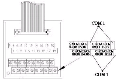
ADAM-5038S Digital Input Wiring
