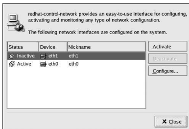
Figure 11-16. Activating Devices
