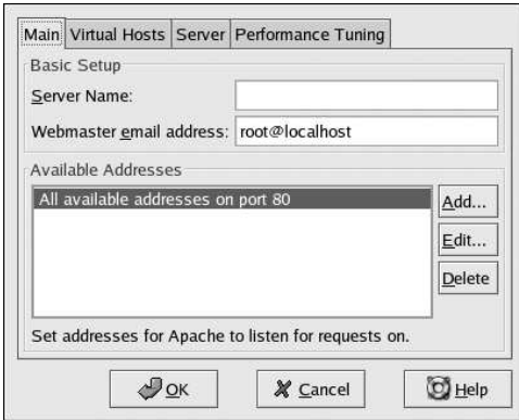
Figure 18-1. Basic Settings
