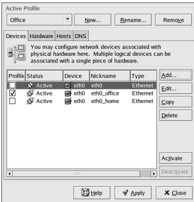
Figure 11-17. Office Profile
