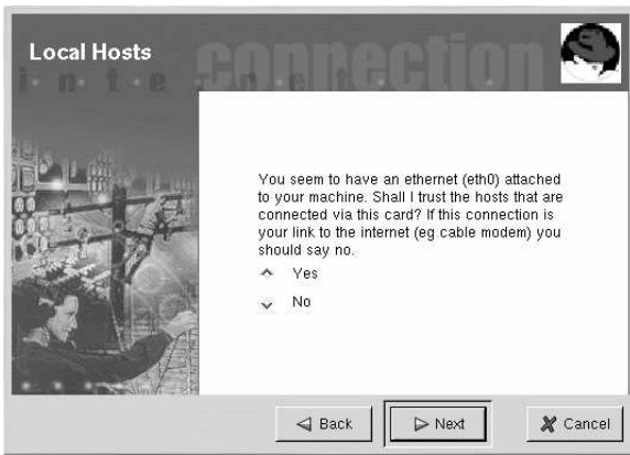
Figure 12-3. Local Hosts
