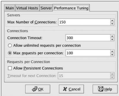
Figure 18-11. Performance Tuning
