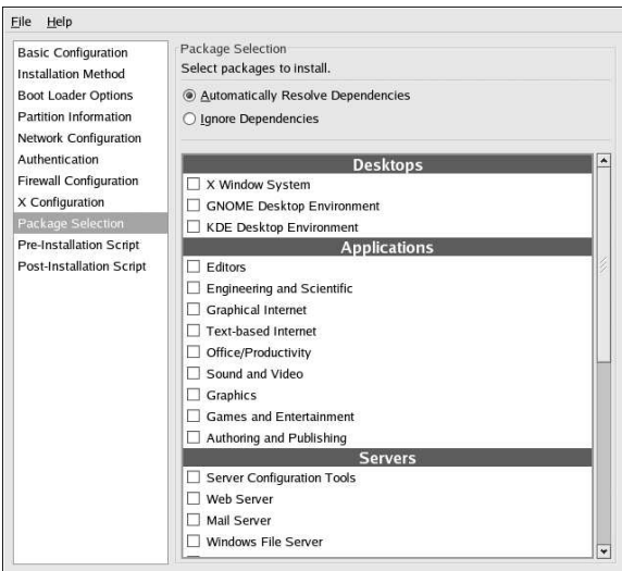
Figure 7-14. Package Selection
