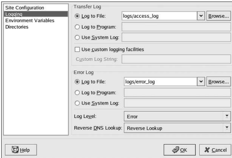
Figure 18-4. Logging
