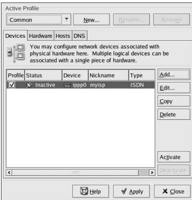
Figure 11-4. ISDN Device
