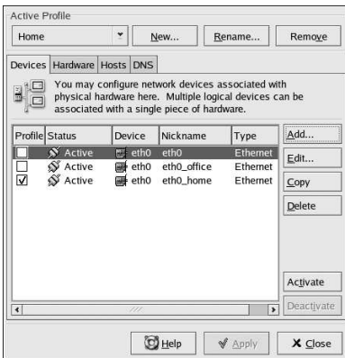
Figure 11-18. Home Profile
