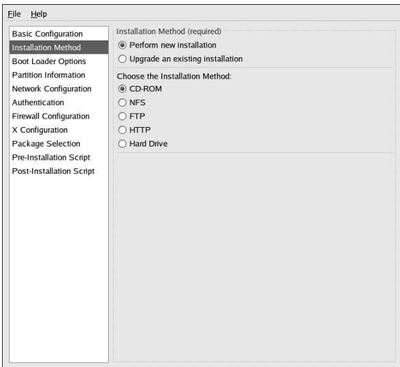
Figure 7-2. Installation Method
