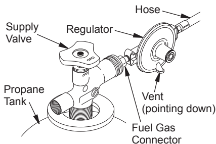
Figure 3 - Regulator With Vent Pointing Down
