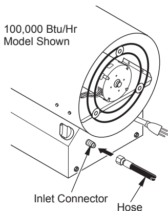
Figure 4 - Hose and Inlet Connector
