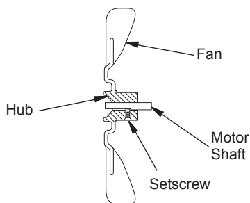
Figure 9 - Fan Cross Section
