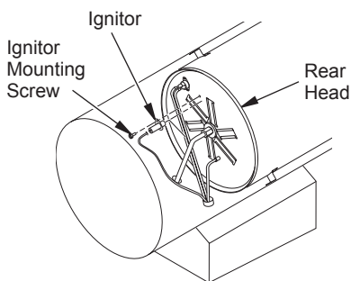
Figure 11 - Removing Ignitor Mounting Screw and Ignitor
