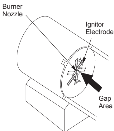
Figure 12 - Clearance between Ignitor Electrode and Target Plate
