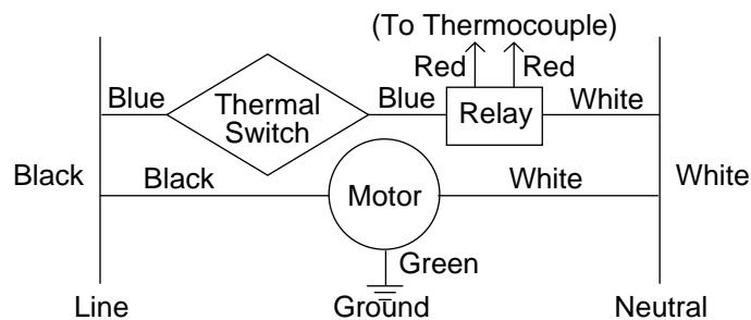
Figure 15 - Electrical Ladder Diagram
