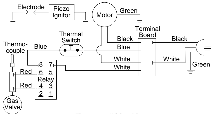
Figure 14 - Wiring Diagram
