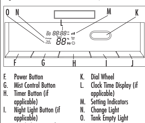
Figure 2 Control Panel (close-up)
